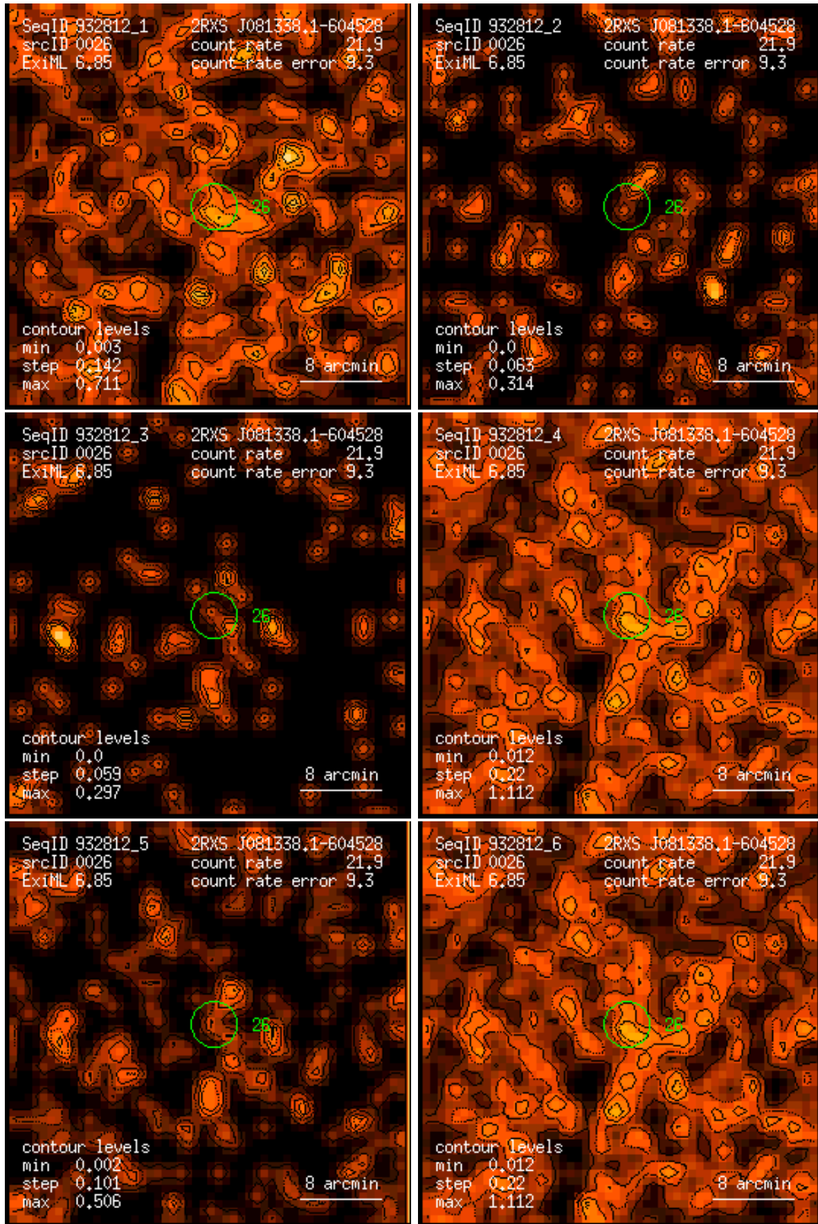
Figure 26: RASS 932812: detection 0026: band rate images, Gaussian filter: (1) PSPC channels 11 – 41, (2) 52 – 90, (3) 91 – 201, (4) 11 – 235, (5) 52 – 201, (6) 11 – 201. Broad band rates in counts/ks. Band rate contour levels in counts/ks/arcmin 2 .
