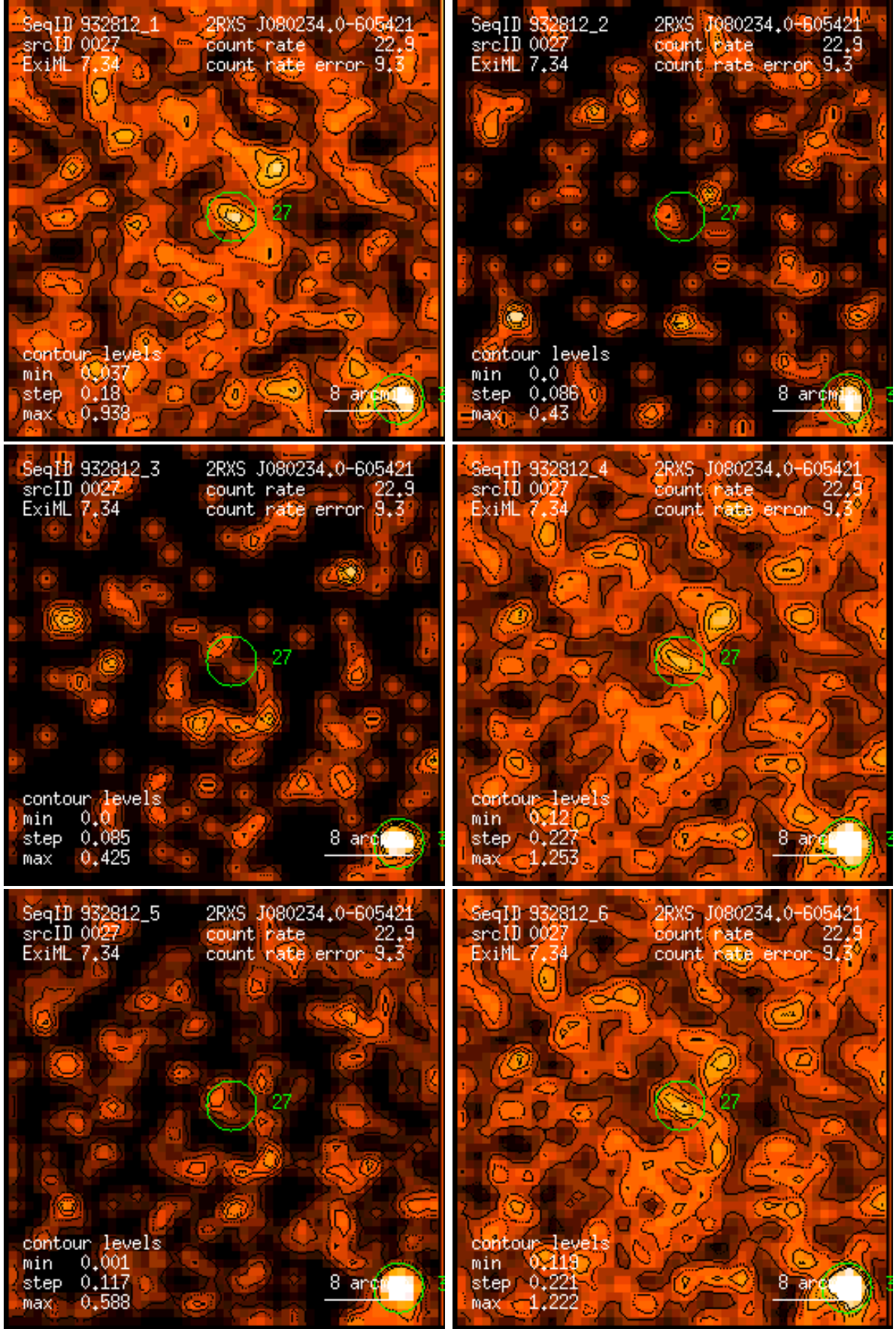
Figure 27: RASS 932812: detection 0027: band rate images, Gaussian filter: (1) PSPC channels 11 – 41, (2) 52 – 90, (3) 91 – 201, (4) 11 – 235, (5) 52 – 201, (6) 11 – 201. Broad band rates in counts/ks. Band rate contour levels in counts/ks/arcmin 2 .
