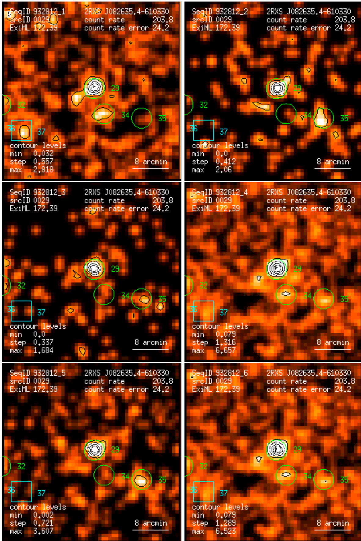
Figure 29: RASS 932812: detection 0029: band rate images, Gaussian filter: (1) PSPC channels 11 – 41, (2) 52 – 90, (3) 91 – 201, (4) 11 – 235, (5) 52 – 201, (6) 11 – 201. Broad band rates in counts/ks. Band rate contour levels in counts/ks/arcmin 2 .
