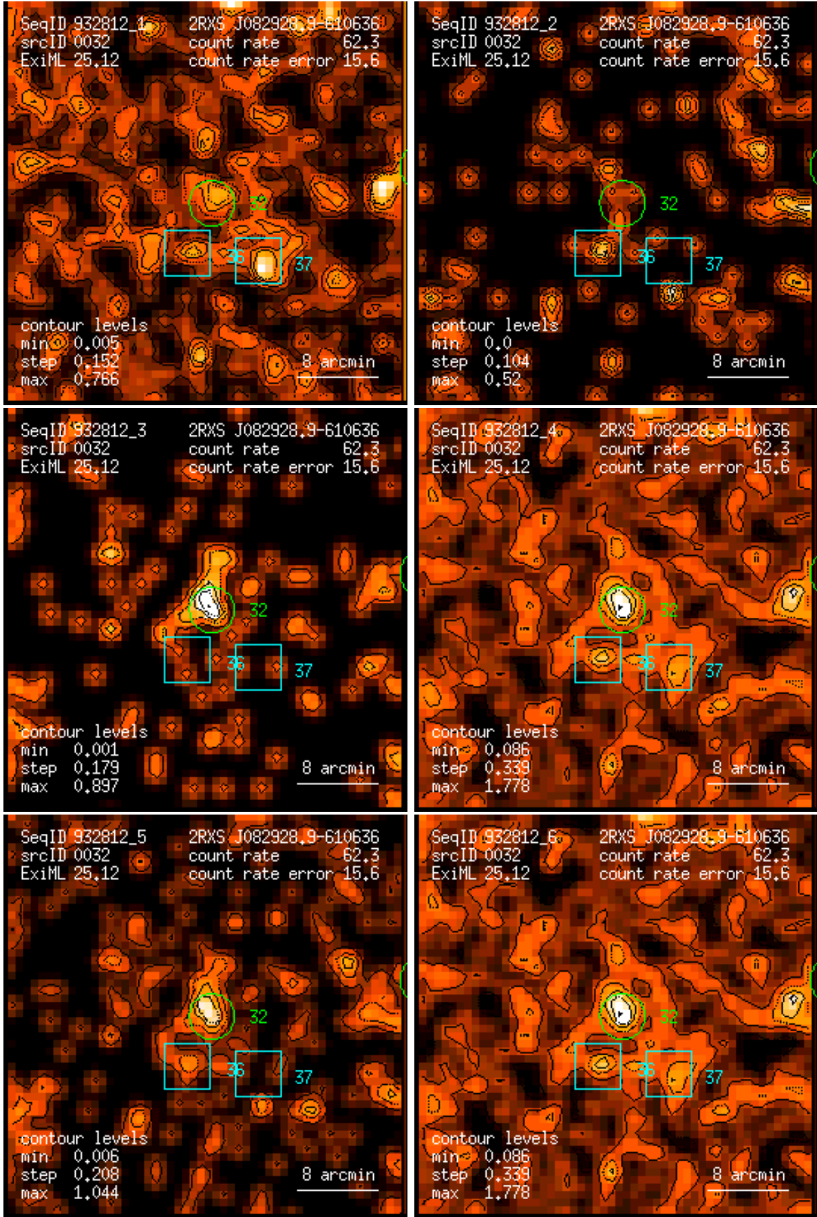
Figure 32: RASS 932812: detection 0032: band rate images, Gaussian filter: (1) PSPC channels 11 – 41, (2) 52 – 90, (3) 91 – 201, (4) 11 – 235, (5) 52 – 201, (6) 11 – 201. Broad band rates in counts/ks. Band rate contour levels in counts/ks/arcmin 2 .
