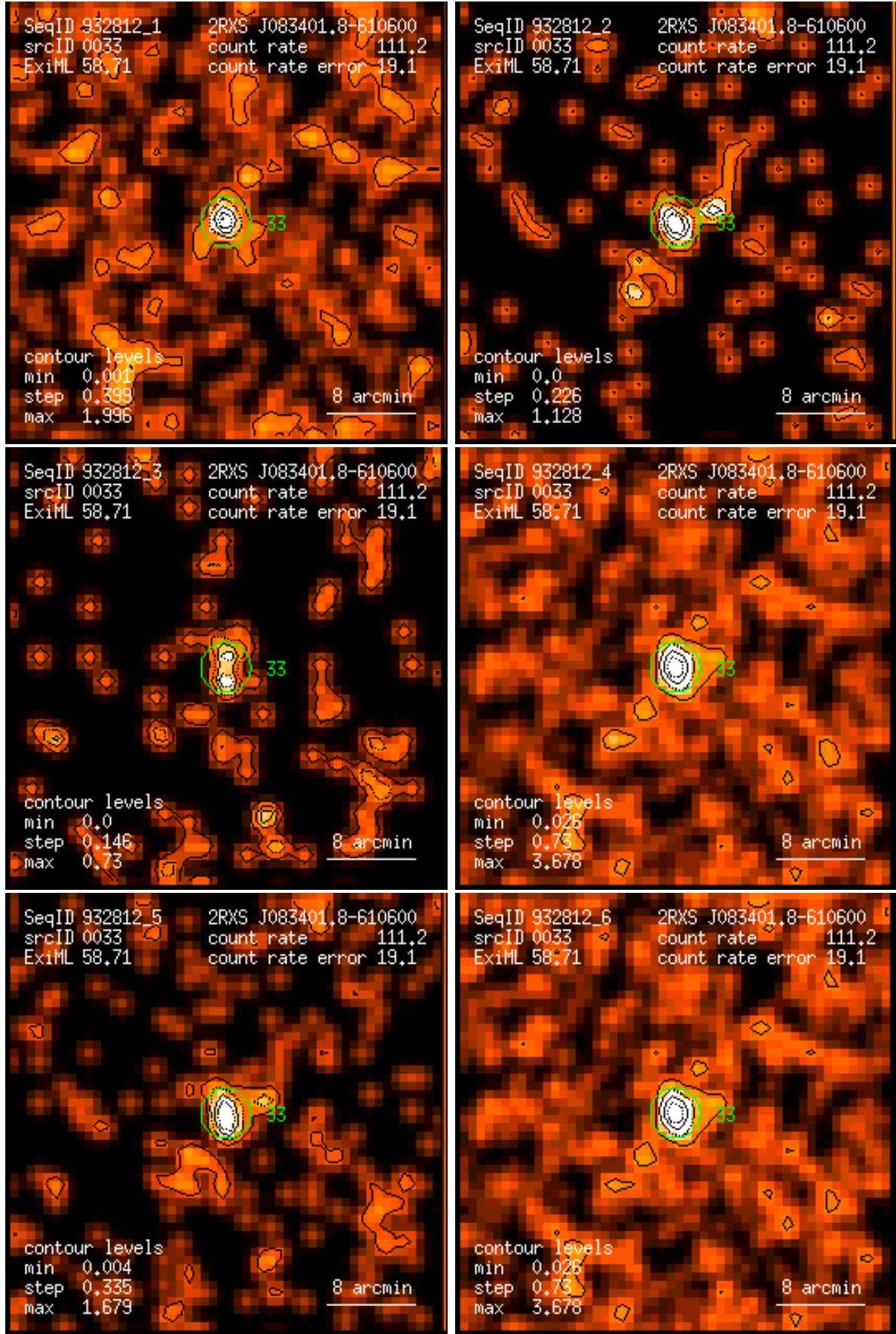
Figure 33: RASS 932812: detection 0033: band rate images, Gaussian filter: (1) PSPC channels 11 – 41, (2) 52 – 90, (3) 91 – 201, (4) 11 – 235, (5) 52 – 201, (6) 11 – 201. Broad band rates in counts/ks. Band rate contour levels in counts/ks/arcmin 2 .
