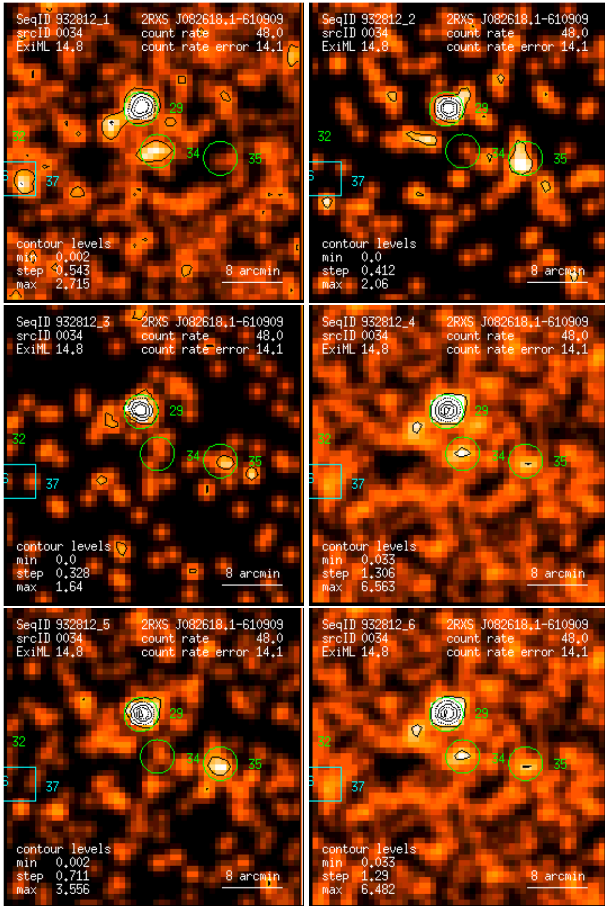
Figure 34: RASS 932812: detection 0034: band rate images, Gaussian filter: (1) PSPC channels 11 – 41, (2) 52 – 90, (3) 91 – 201, (4) 11 – 235, (5) 52 – 201, (6) 11 – 201. Broad band rates in counts/ks. Band rate contour levels in counts/ks/arcmin 2 .
