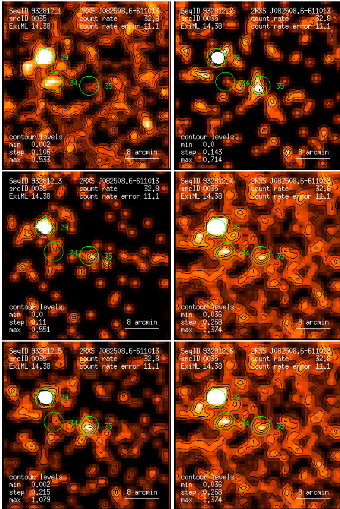
Figure 35: RASS 932812: detection 0035: band rate images, Gaussian filter: (1) PSPC channels 11 – 41, (2) 52 – 90, (3) 91 – 201, (4) 11 – 235, (5) 52 – 201, (6) 11 – 201. Broad band rates in counts/ks. Band rate contour levels in counts/ks/arcmin 2 .
