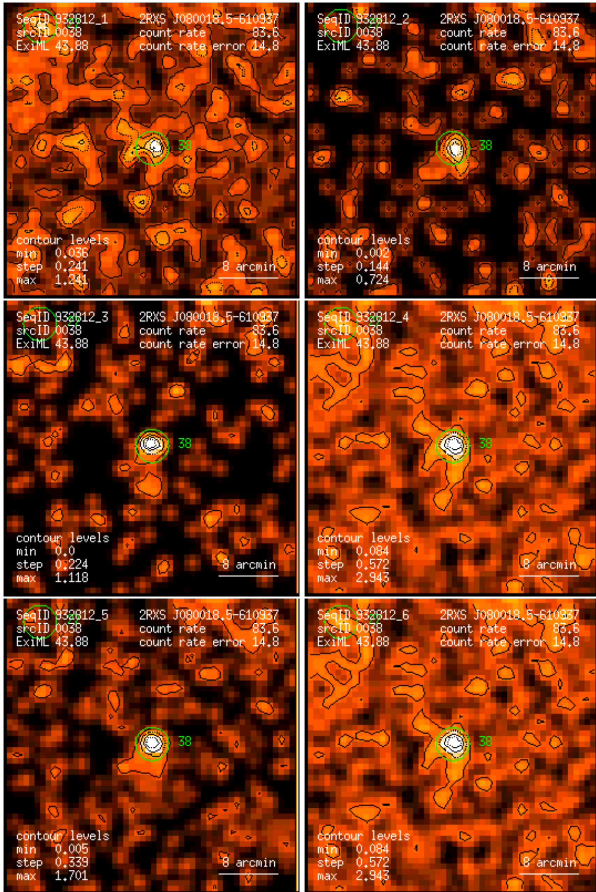
Figure 38: RASS 932812: detection 0038: band rate images, Gaussian filter: (1) PSPC channels 11 – 41, (2) 52 – 90, (3) 91 – 201, (4) 11 – 235, (5) 52 – 201, (6) 11 – 201. Broad band rates in counts/ks. Band rate contour levels in counts/ks/arcmin 2 .
