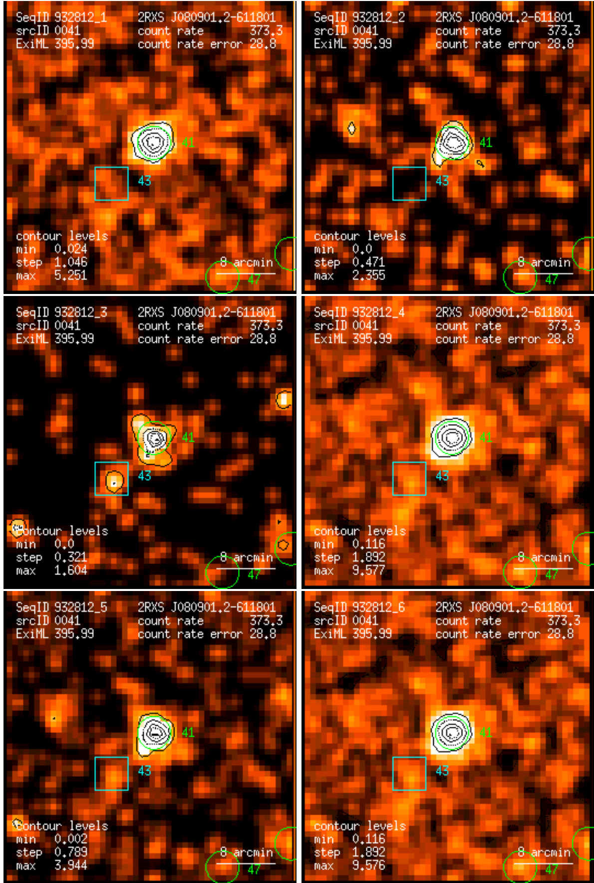
Figure 41: RASS 932812: detection 0041: band rate images, Gaussian filter: (1) PSPC channels 11 – 41, (2) 52 – 90, (3) 91 – 201, (4) 11 – 235, (5) 52 – 201, (6) 11 – 201. Broad band rates in counts/ks. Band rate contour levels in counts/ks/arcmin 2 .
