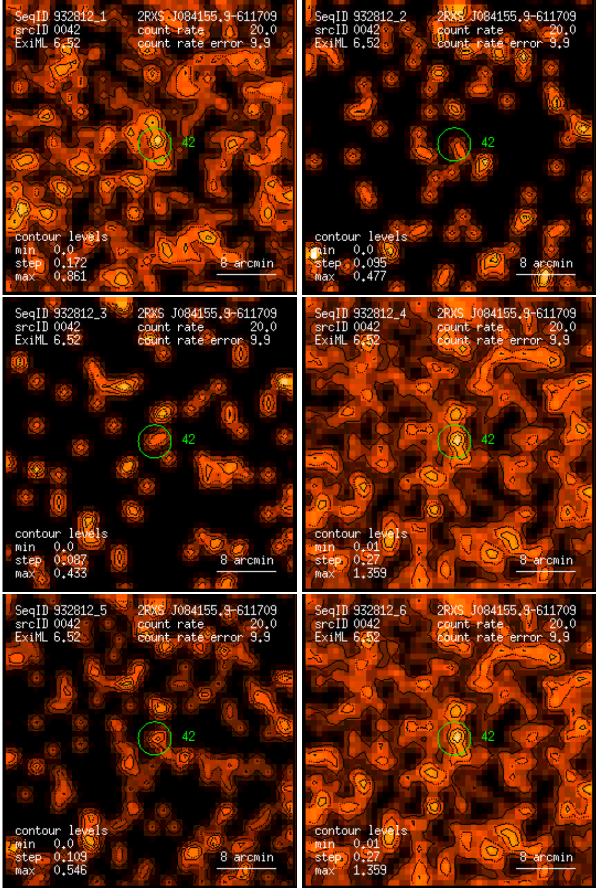
Figure 42: RASS 932812: detection 0042: band rate images, Gaussian filter: (1) PSPC channels 11 – 41, (2) 52 – 90, (3) 91 – 201, (4) 11 – 235, (5) 52 – 201, (6) 11 – 201. Broad band rates in counts/ks. Band rate contour levels in counts/ks/arcmin 2 .
