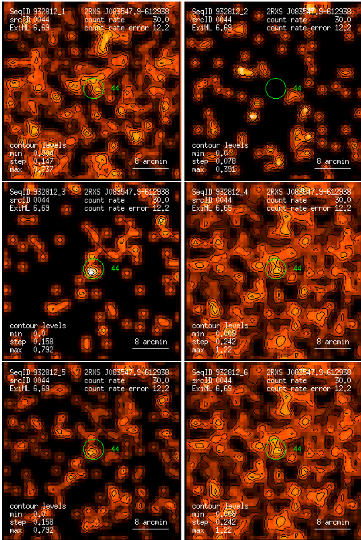
Figure 44: RASS 932812: detection 0044: band rate images, Gaussian filter: (1) PSPC channels 11 – 41, (2) 52 – 90, (3) 91 – 201, (4) 11 – 235, (5) 52 – 201, (6) 11 – 201. Broad band rates in counts/ks. Band rate contour levels in counts/ks/arcmin 2 .
