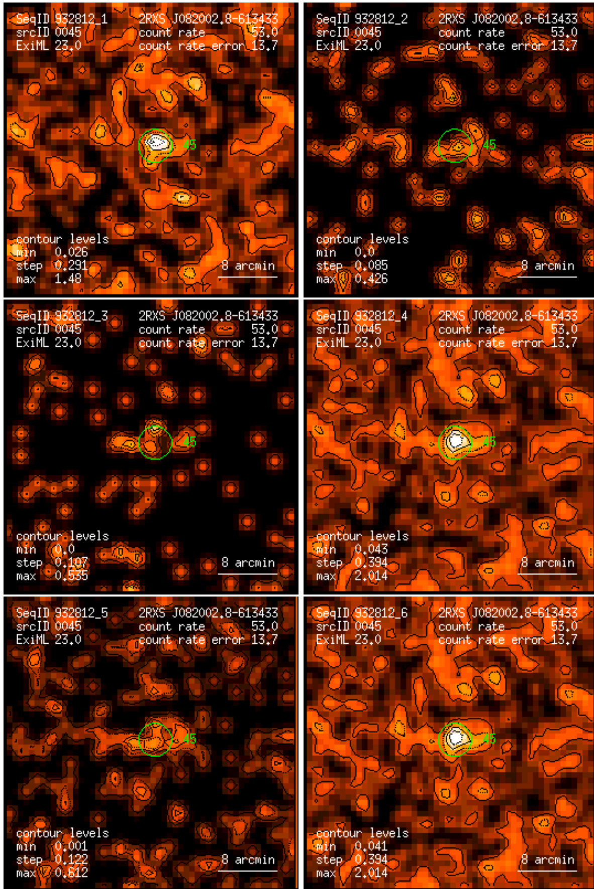
Figure 45: RASS 932812: detection 0045: band rate images, Gaussian filter: (1) PSPC channels 11 – 41, (2) 52 – 90, (3) 91 – 201, (4) 11 – 235, (5) 52 – 201, (6) 11 – 201. Broad band rates in counts/ks. Band rate contour levels in counts/ks/arcmin 2 .
