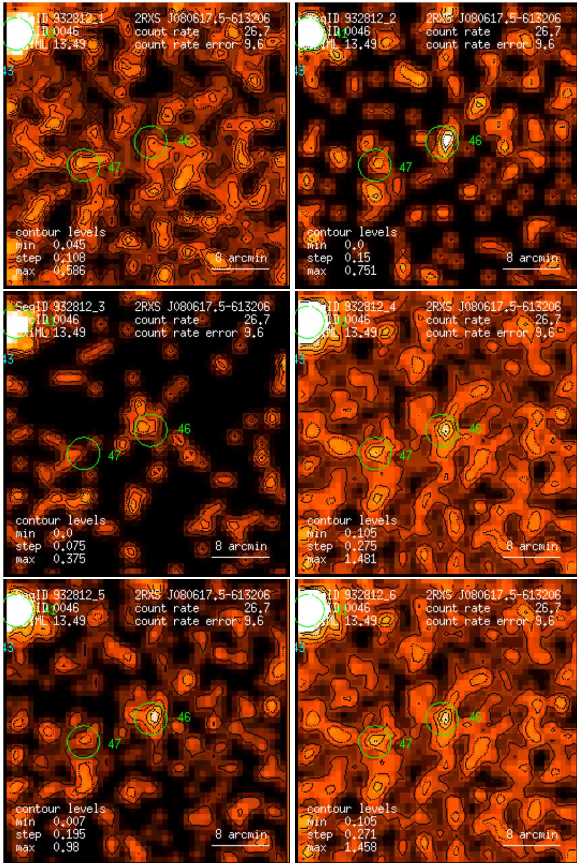
Figure 46: RASS 932812: detection 0046: band rate images, Gaussian filter: (1) PSPC channels 11 – 41, (2) 52 – 90, (3) 91 – 201, (4) 11 – 235, (5) 52 – 201, (6) 11 – 201. Broad band rates in counts/ks. Band rate contour levels in counts/ks/arcmin 2 .
