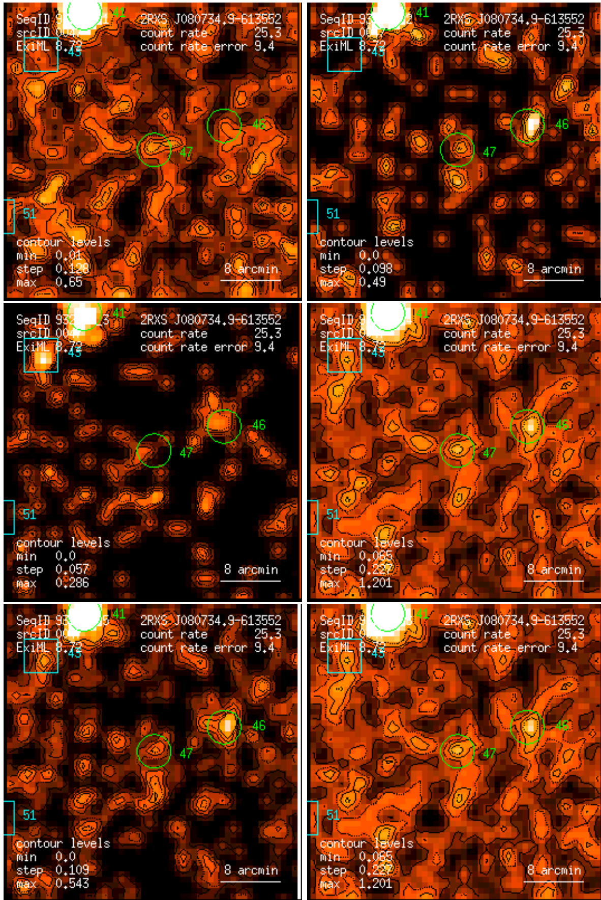
Figure 47: RASS 932812: detection 0047: band rate images, Gaussian filter: (1) PSPC channels 11 – 41, (2) 52 – 90, (3) 91 – 201, (4) 11 – 235, (5) 52 – 201, (6) 11 – 201. Broad band rates in counts/ks. Band rate contour levels in counts/ks/arcmin 2 .
