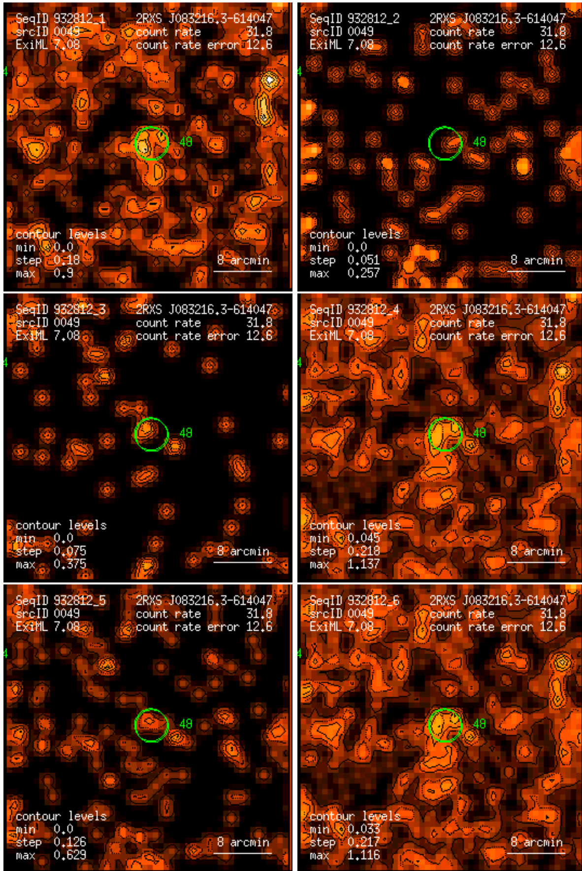
Figure 49: RASS 932812: detection 0049: band rate images, Gaussian filter: (1) PSPC channels 11 – 41, (2) 52 – 90, (3) 91 – 201, (4) 11 – 235, (5) 52 – 201, (6) 11 – 201. Broad band rates in counts/ks. Band rate contour levels in counts/ks/arcmin 2 .
