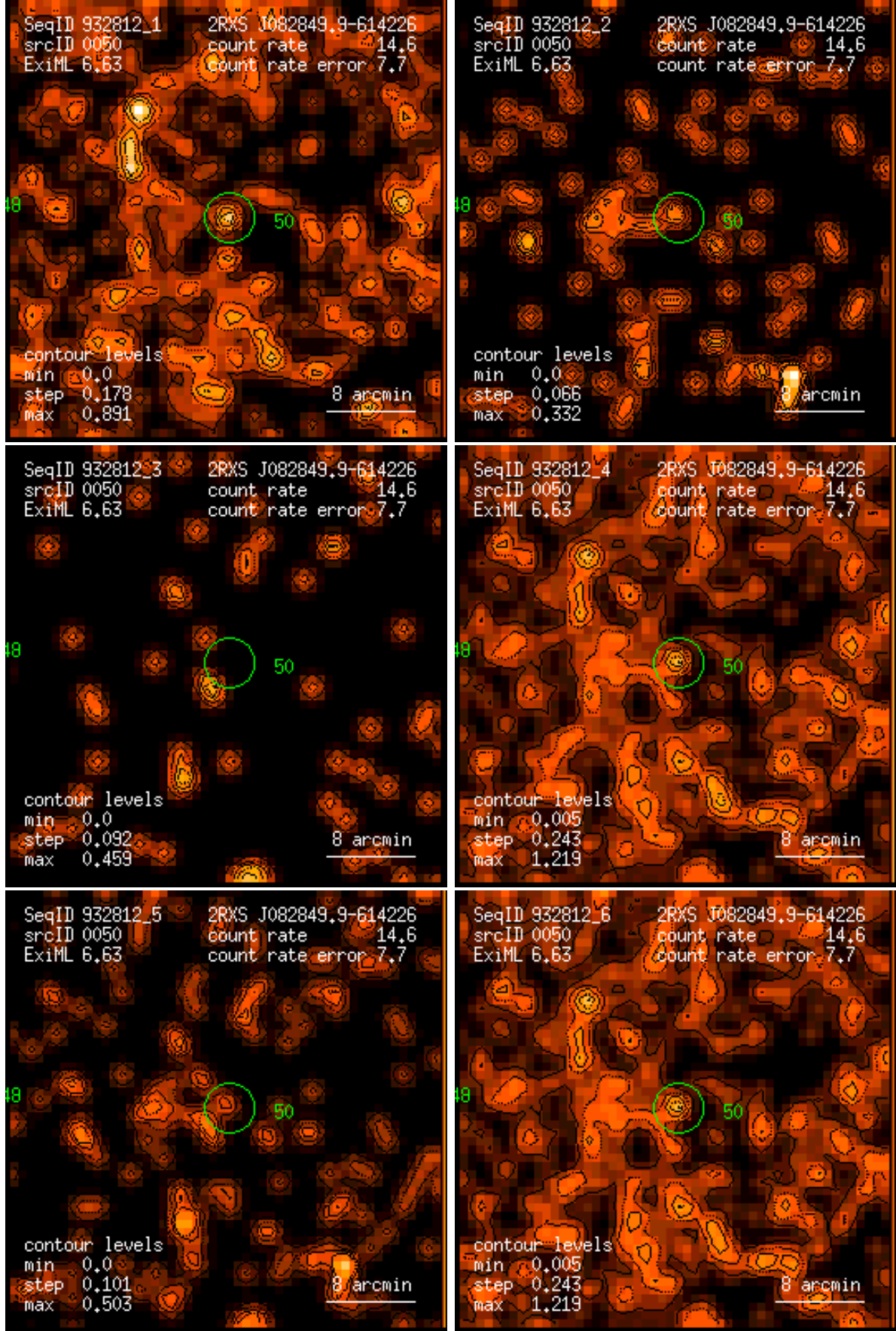
Figure 50: RASS 932812: detection 0050: band rate images, Gaussian filter: (1) PSPC channels 11 – 41, (2) 52 – 90, (3) 91 – 201, (4) 11 – 235, (5) 52 – 201, (6) 11 – 201. Broad band rates in counts/ks. Band rate contour levels in counts/ks/arcmin 2 .
