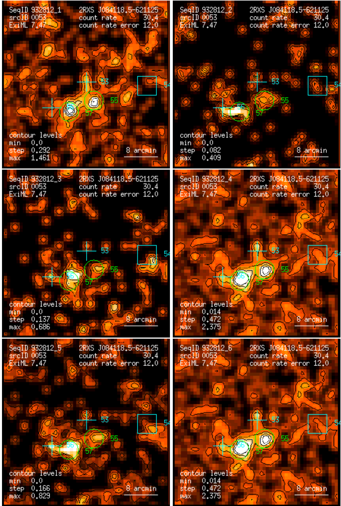
Figure 53: RASS 932812: detection 0053: band rate images, Gaussian filter: (1) PSPC channels 11 – 41, (2) 52 – 90, (3) 91 – 201, (4) 11 – 235, (5) 52 – 201, (6) 11 – 201. Broad band rates in counts/ks. Band rate contour levels in counts/ks/arcmin 2 .
