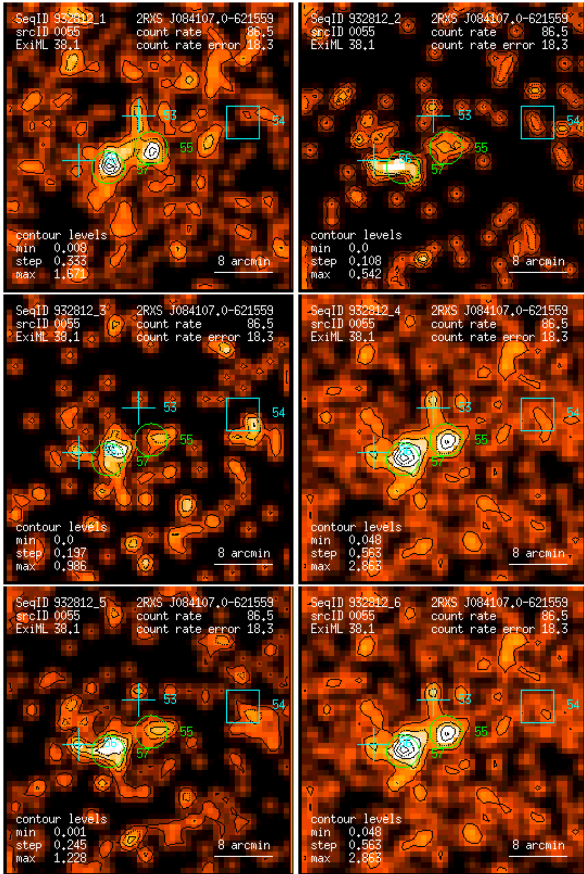
Figure 55: RASS 932812: detection 0055: band rate images, Gaussian filter: (1) PSPC channels 11 – 41, (2) 52 – 90, (3) 91 – 201, (4) 11 – 235, (5) 52 – 201, (6) 11 – 201. Broad band rates in counts/ks. Band rate contour levels in counts/ks/arcmin 2 .
