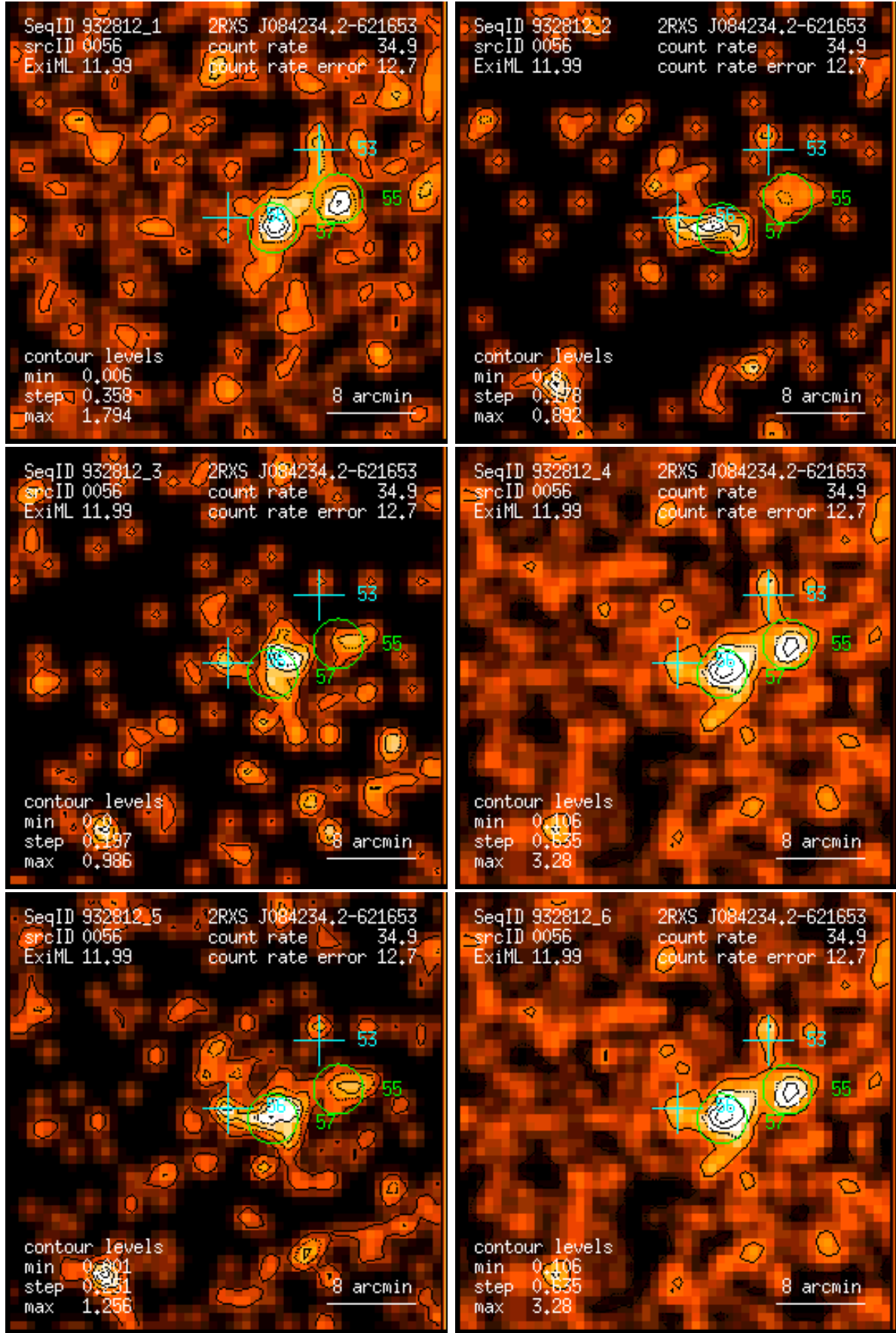
Figure 56: RASS 932812: detection 0056: band rate images, Gaussian filter: (1) PSPC channels 11 – 41, (2) 52 – 90, (3) 91 – 201, (4) 11 – 235, (5) 52 – 201, (6) 11 – 201. Broad band rates in counts/ks. Band rate contour levels in counts/ks/arcmin 2 .
