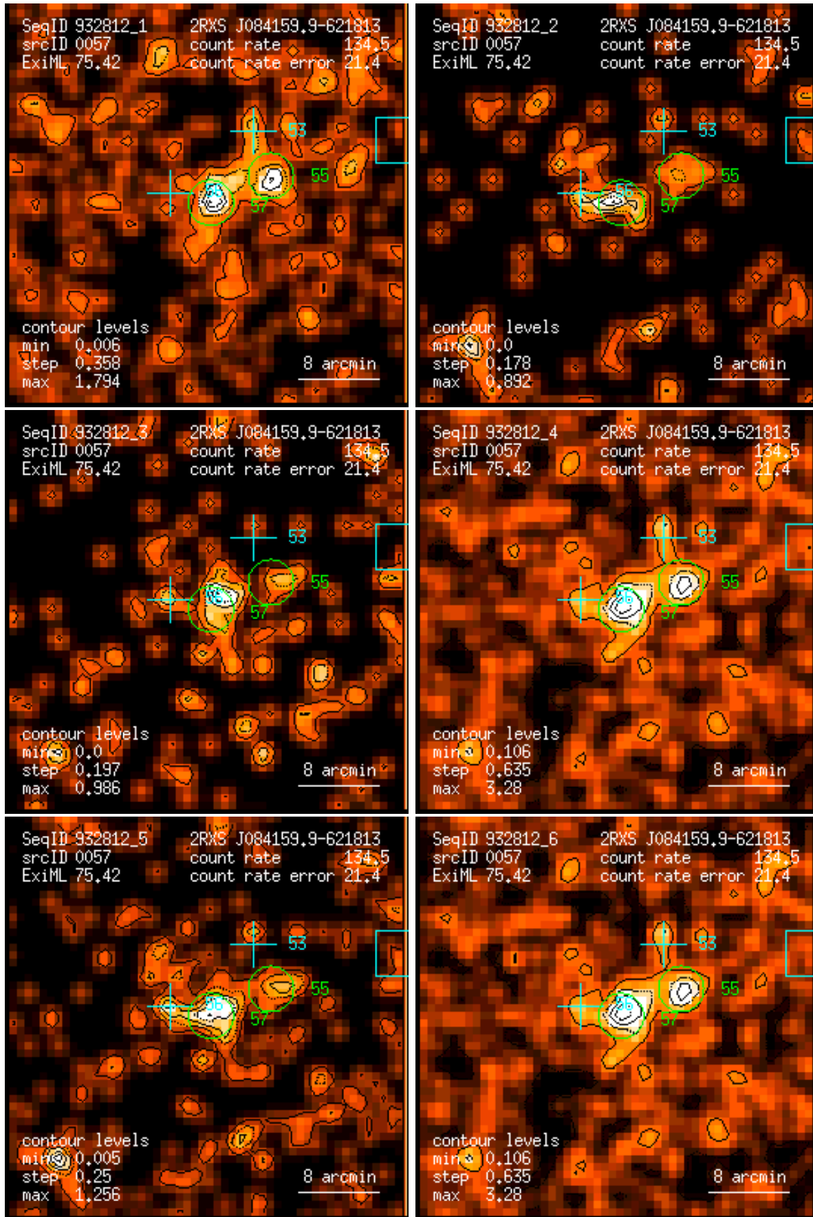
Figure 57: RASS 932812: detection 0057: band rate images, Gaussian filter: (1) PSPC channels 11 – 41, (2) 52 – 90, (3) 91 – 201, (4) 11 – 235, (5) 52 – 201, (6) 11 – 201. Broad band rates in counts/ks. Band rate contour levels in counts/ks/arcmin 2 .
