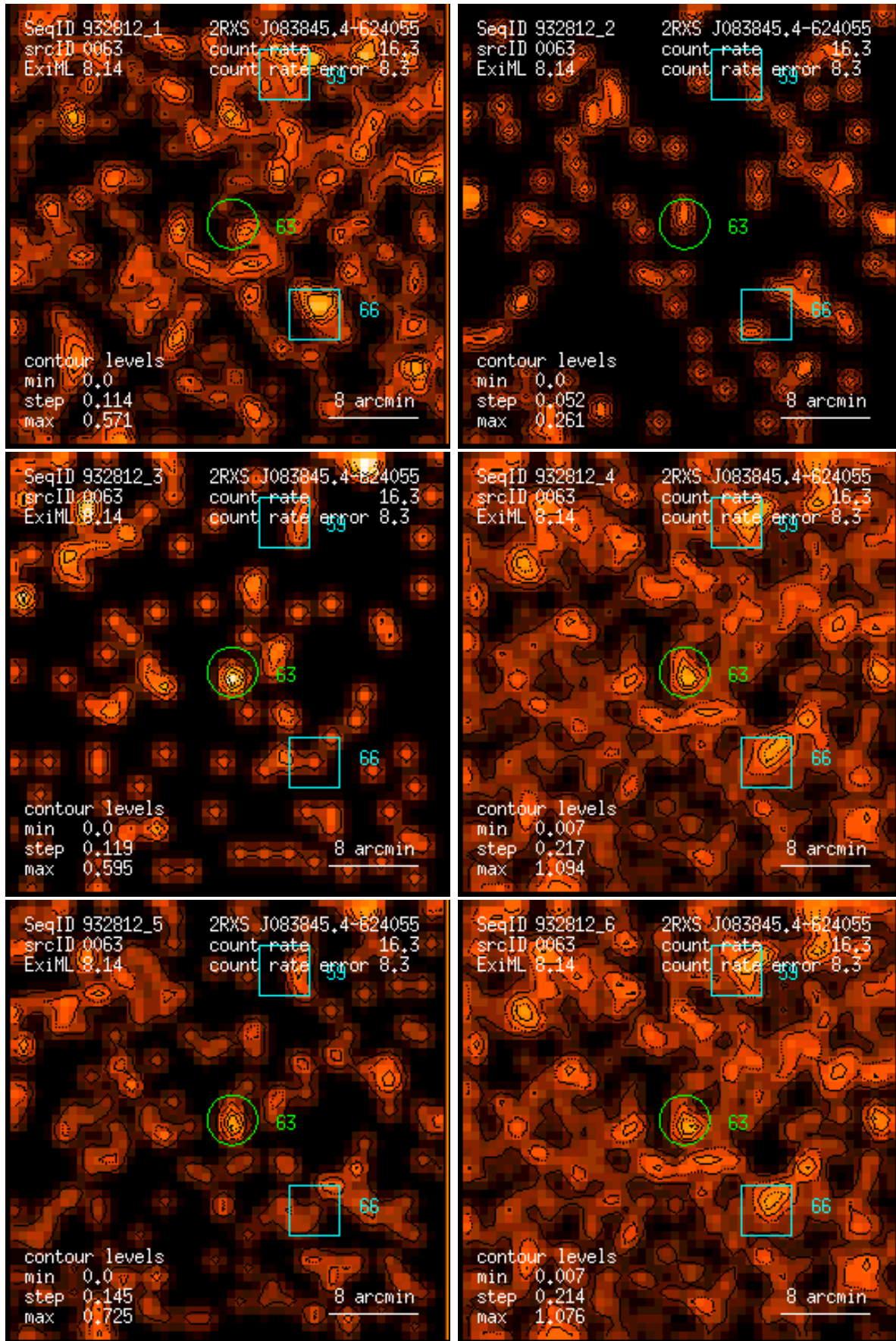
Figure 63: RASS 932812: detection 0063: band rate images, Gaussian filter: (1) PSPC channels 11 – 41, (2) 52 – 90, (3) 91 – 201, (4) 11 – 235, (5) 52 – 201, (6) 11 – 201. Broad band rates in counts/ks. Band rate contour levels in counts/ks/arcmin 2 .
