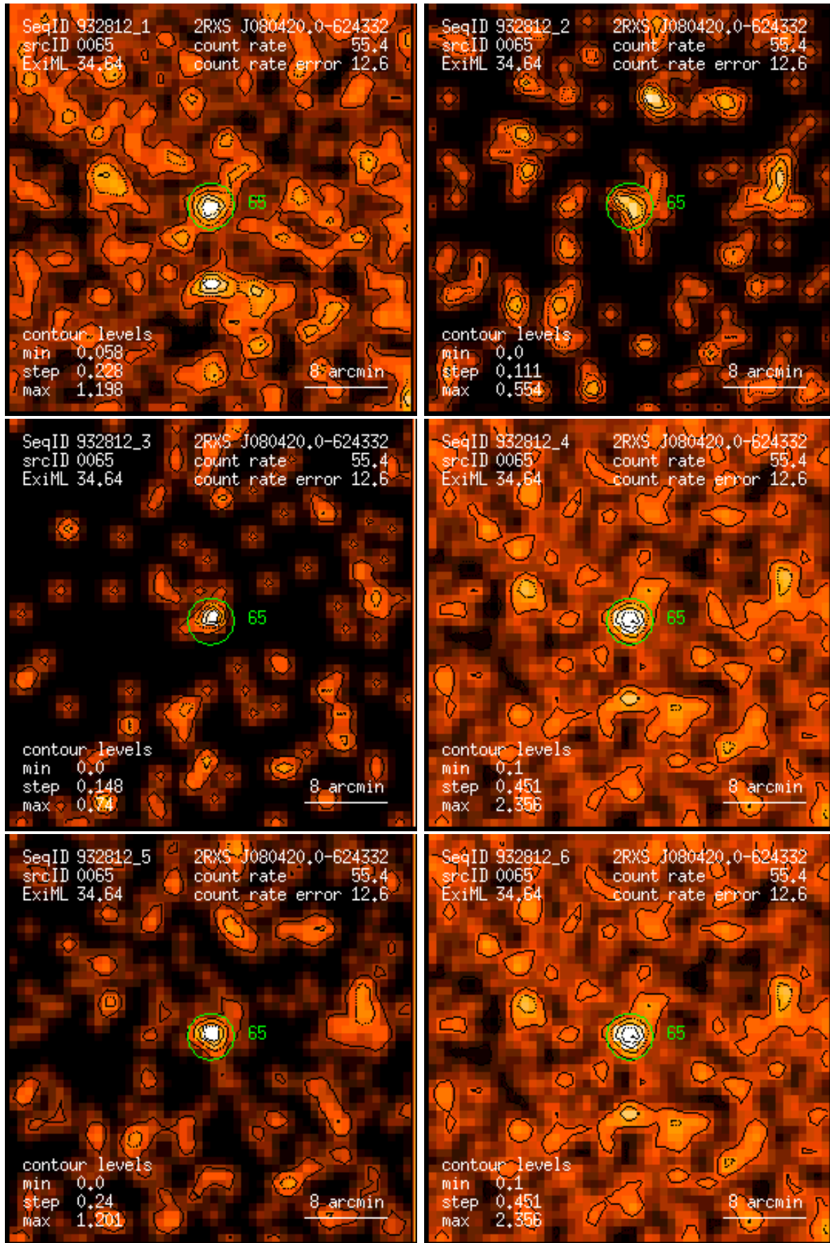
Figure 65: RASS 932812: detection 0065: band rate images, Gaussian filter: (1) PSPC channels 11 – 41, (2) 52 – 90, (3) 91 – 201, (4) 11 – 235, (5) 52 – 201, (6) 11 – 201. Broad band rates in counts/ks. Band rate contour levels in counts/ks/arcmin 2 .
