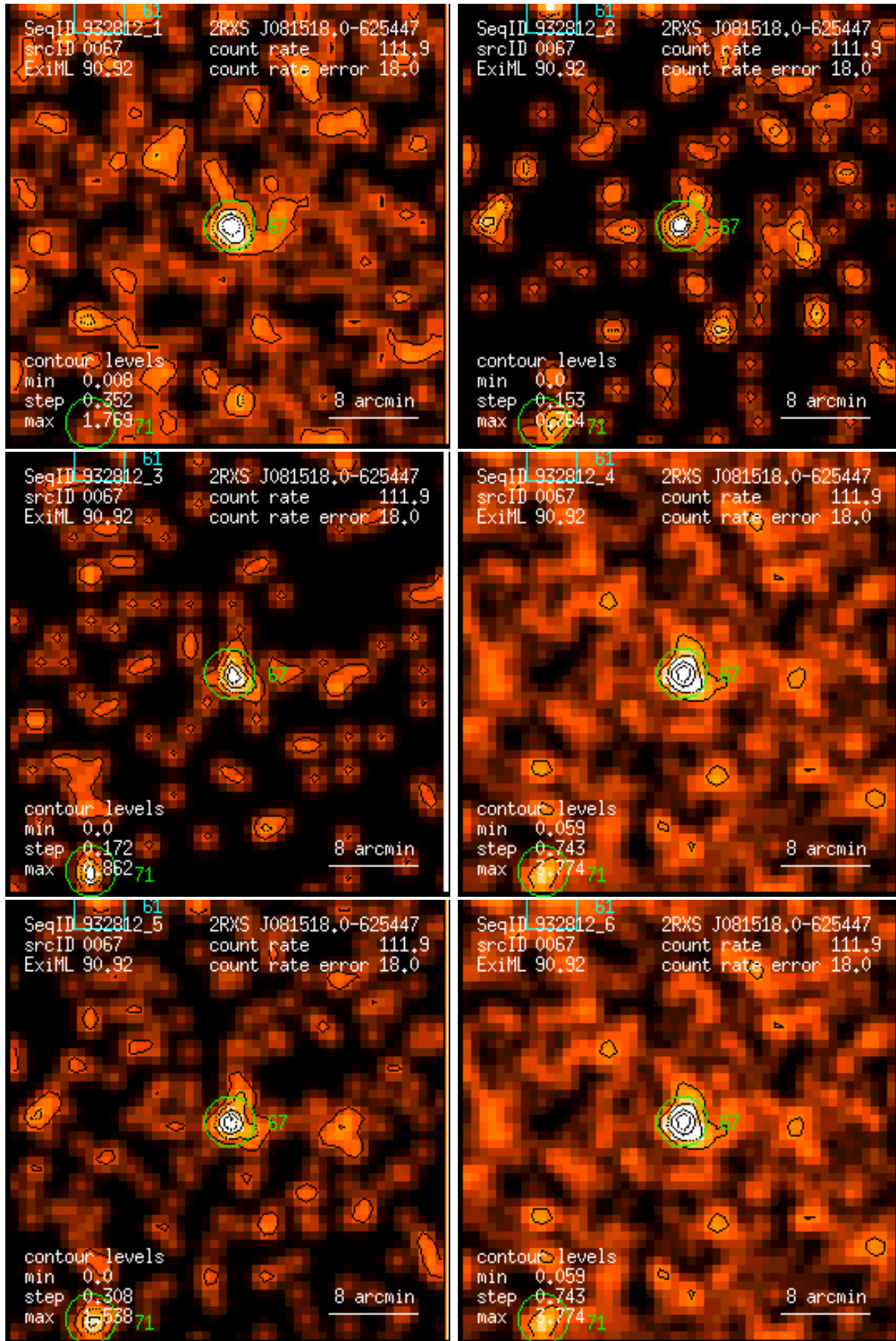
Figure 67: RASS 932812: detection 0067: band rate images, Gaussian filter: (1) PSPC channels 11 – 41, (2) 52 – 90, (3) 91 – 201, (4) 11 – 235, (5) 52 – 201, (6) 11 – 201. Broad band rates in counts/ks. Band rate contour levels in counts/ks/arcmin 2 .
