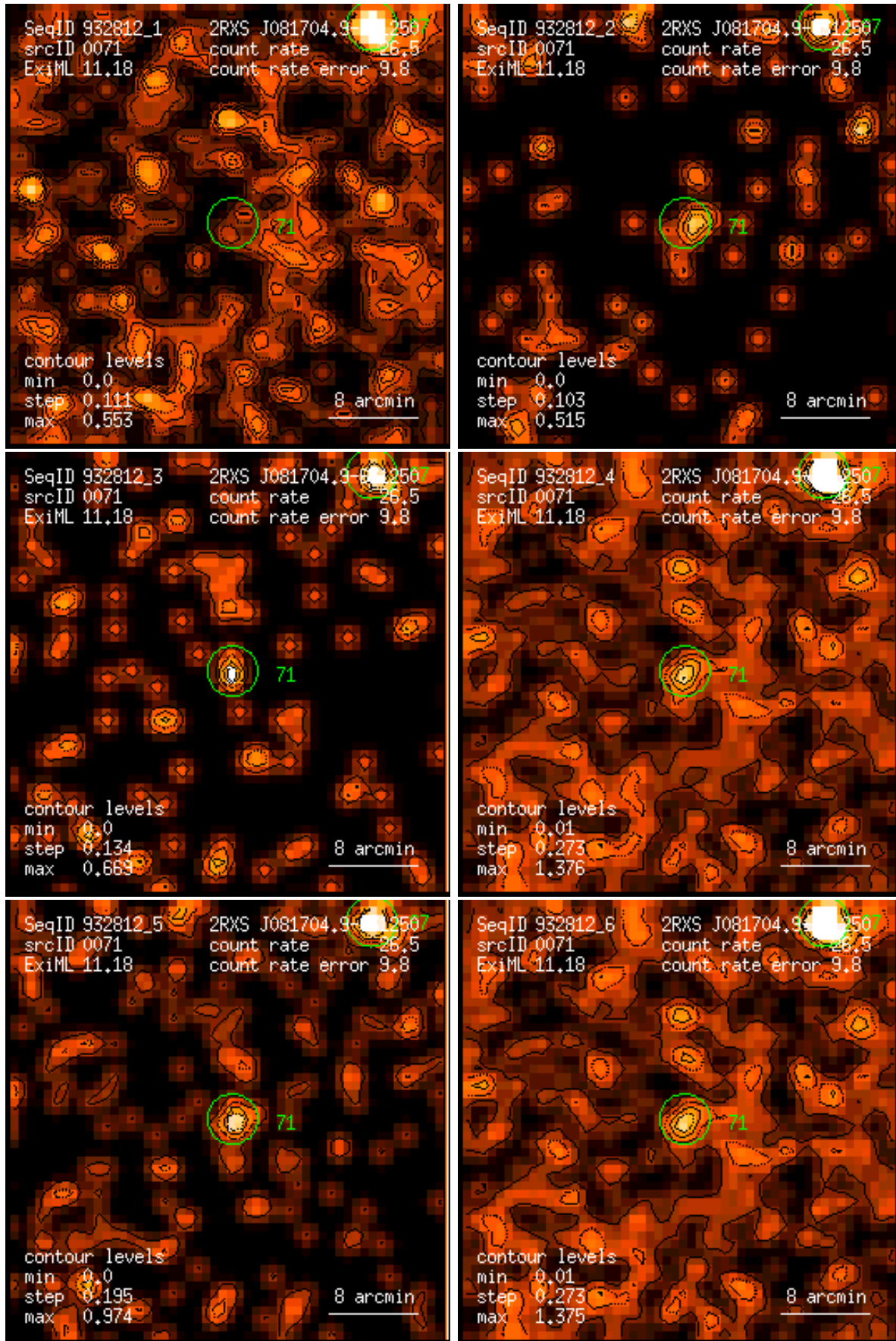
Figure 71: RASS 932812: detection 0071: band rate images, Gaussian filter: (1) PSPC channels 11 – 41, (2) 52 – 90, (3) 91 – 201, (4) 11 – 235, (5) 52 – 201, (6) 11 – 201. Broad band rates in counts/ks. Band rate contour levels in counts/ks/arcmin 2 .
