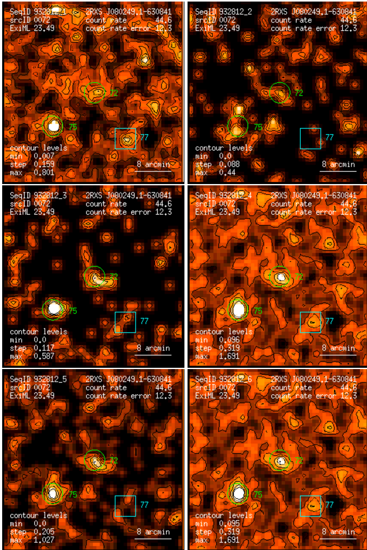
Figure 72: RASS 932812: detection 0072: band rate images, Gaussian filter: (1) PSPC channels 11 – 41, (2) 52 – 90, (3) 91 – 201, (4) 11 – 235, (5) 52 – 201, (6) 11 – 201. Broad band rates in counts/ks. Band rate contour levels in counts/ks/arcmin 2 .
