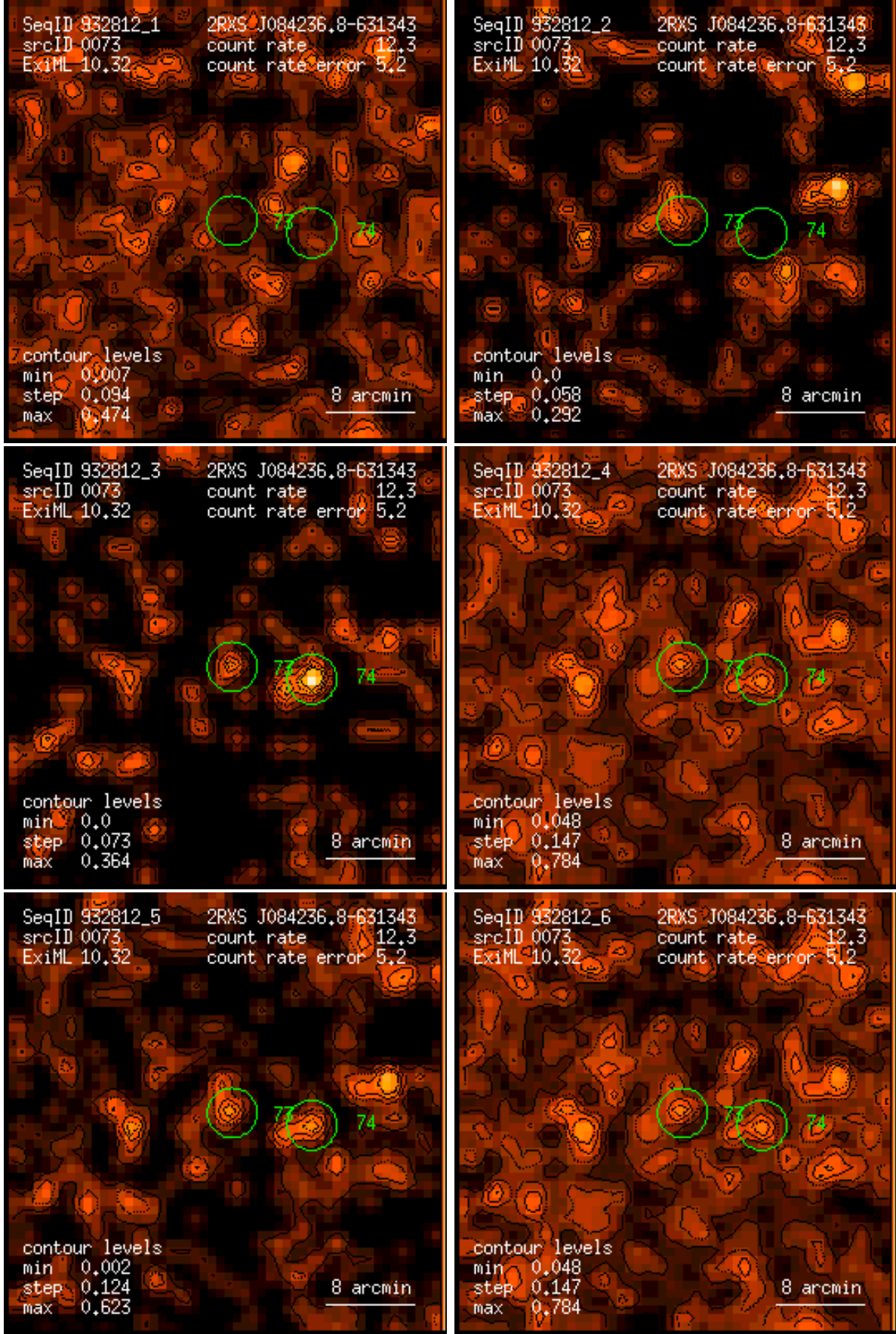
Figure 73: RASS 932812: detection 0073: band rate images, Gaussian filter: (1) PSPC channels 11 – 41, (2) 52 – 90, (3) 91 – 201, (4) 11 – 235, (5) 52 – 201, (6) 11 – 201. Broad band rates in counts/ks. Band rate contour levels in counts/ks/arcmin 2 .
