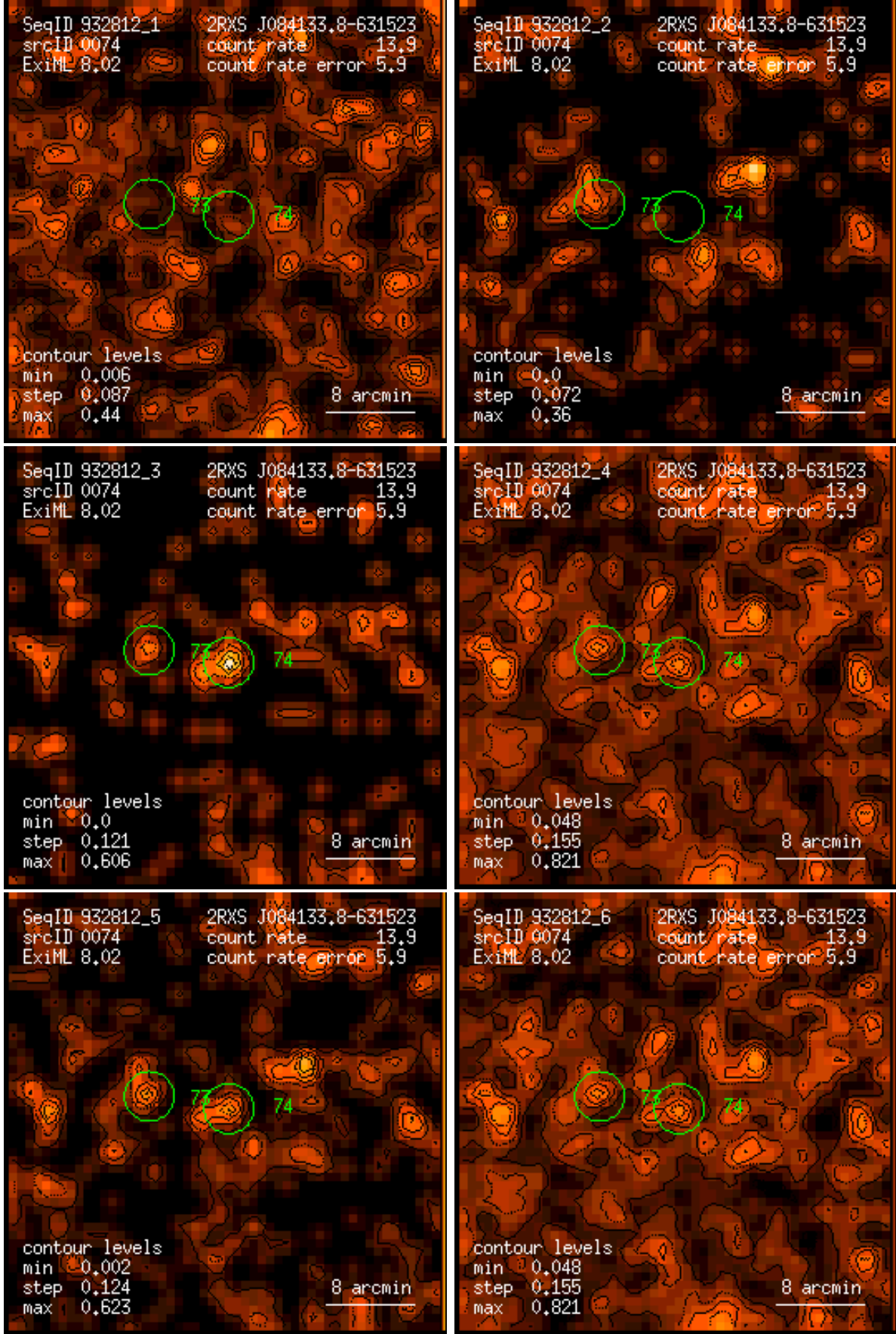
Figure 74: RASS 932812: detection 0074: band rate images, Gaussian filter: (1) PSPC channels 11 – 41, (2) 52 – 90, (3) 91 – 201, (4) 11 – 235, (5) 52 – 201, (6) 11 – 201. Broad band rates in counts/ks. Band rate contour levels in counts/ks/arcmin 2 .
