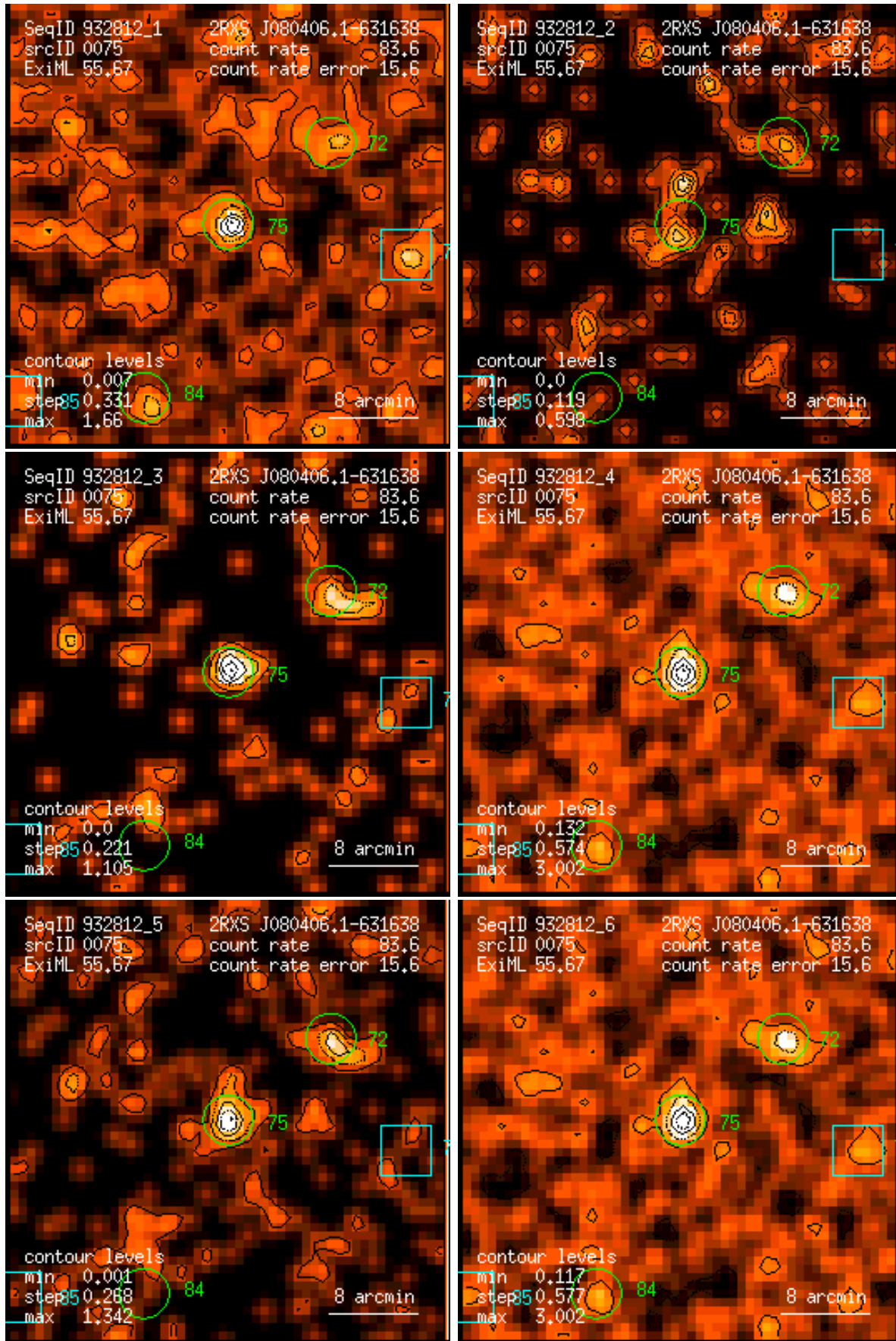
Figure 75: RASS 932812: detection 0075: band rate images, Gaussian filter: (1) PSPC channels 11 – 41, (2) 52 – 90, (3) 91 – 201, (4) 11 – 235, (5) 52 – 201, (6) 11 – 201. Broad band rates in counts/ks. Band rate contour levels in counts/ks/arcmin 2 .
