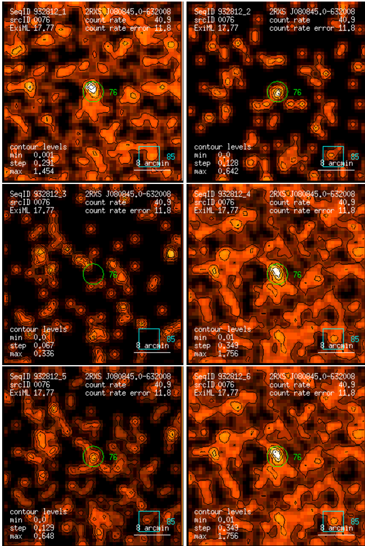
Figure 76: RASS 932812: detection 0076: band rate images, Gaussian filter: (1) PSPC channels 11 – 41, (2) 52 – 90, (3) 91 – 201, (4) 11 – 235, (5) 52 – 201, (6) 11 – 201. Broad band rates in counts/ks. Band rate contour levels in counts/ks/arcmin 2 .
