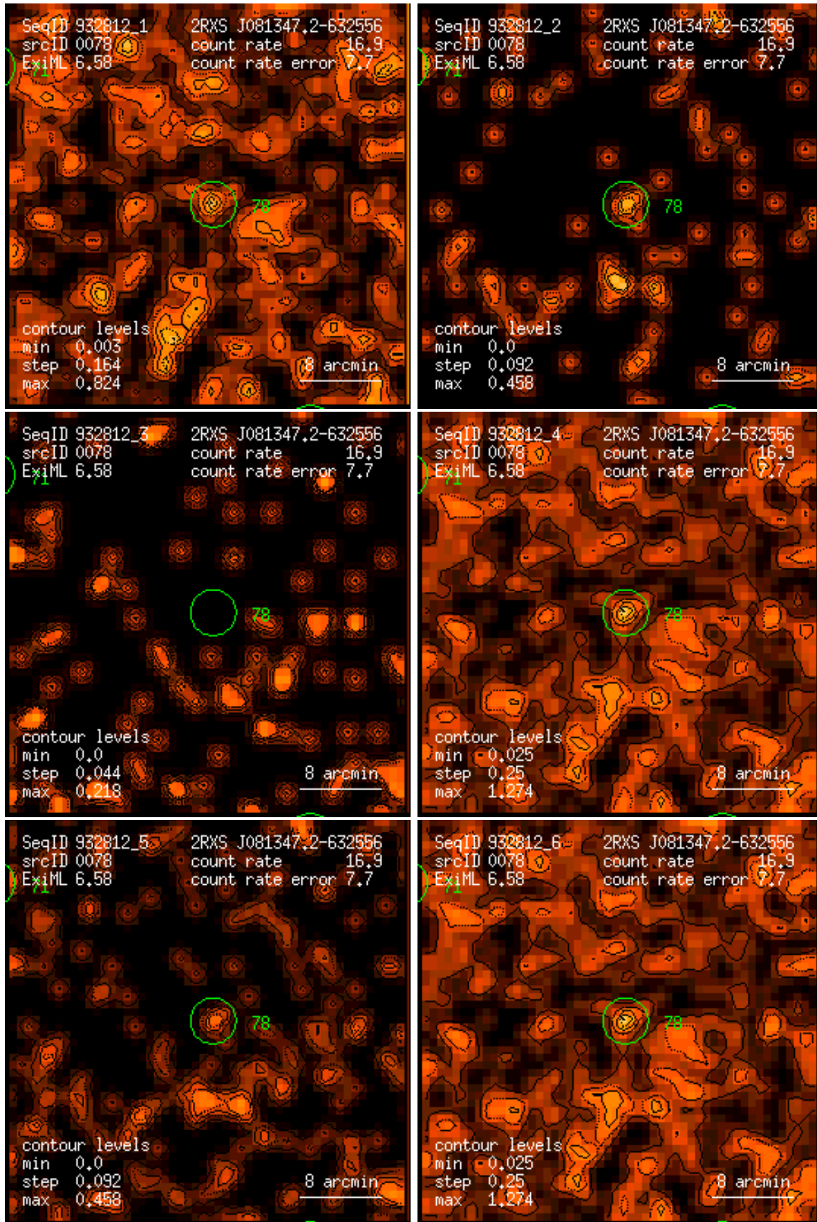
Figure 78: RASS 932812: detection 0078: band rate images, Gaussian filter: (1) PSPC channels 11 – 41, (2) 52 – 90, (3) 91 – 201, (4) 11 – 235, (5) 52 – 201, (6) 11 – 201. Broad band rates in counts/ks. Band rate contour levels in counts/ks/arcmin 2 .
