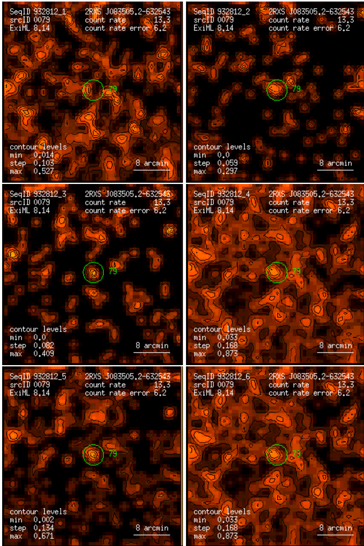
Figure 79: RASS 932812: detection 0079: band rate images, Gaussian filter: (1) PSPC channels 11 – 41, (2) 52 – 90, (3) 91 – 201, (4) 11 – 235, (5) 52 – 201, (6) 11 – 201. Broad band rates in counts/ks. Band rate contour levels in counts/ks/arcmin 2 .
