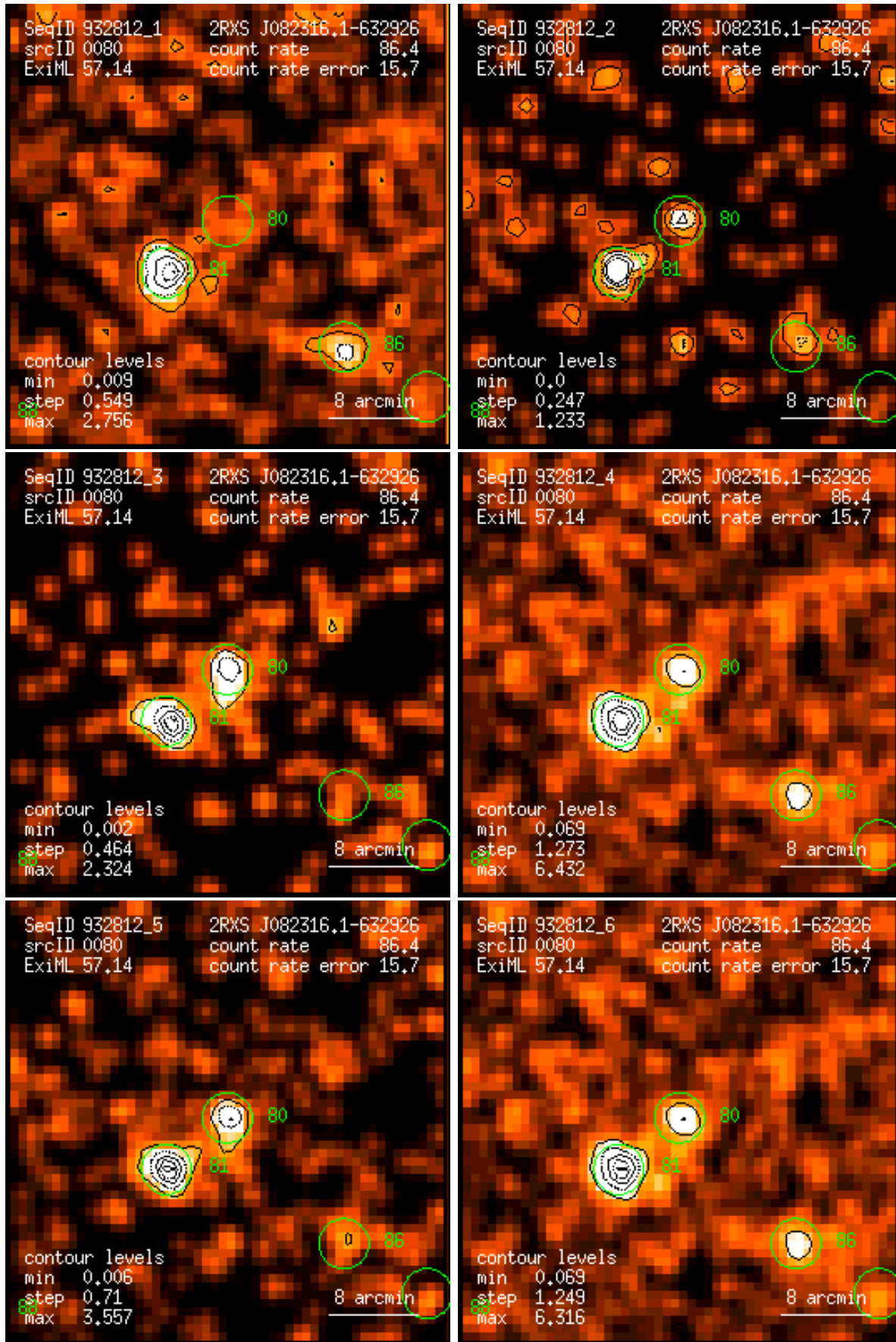
Figure 80: RASS 932812: detection 0080: band rate images, Gaussian filter: (1) PSPC channels 11 – 41, (2) 52 – 90, (3) 91 – 201, (4) 11 – 235, (5) 52 – 201, (6) 11 – 201. Broad band rates in counts/ks. Band rate contour levels in counts/ks/arcmin 2 .
