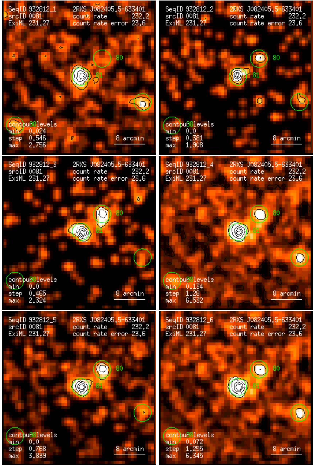
Figure 81: RASS 932812: detection 0081: band rate images, Gaussian filter: (1) PSPC channels 11 – 41, (2) 52 – 90, (3) 91 – 201, (4) 11 – 235, (5) 52 – 201, (6) 11 – 201. Broad band rates in counts/ks. Band rate contour levels in counts/ks/arcmin 2 .
