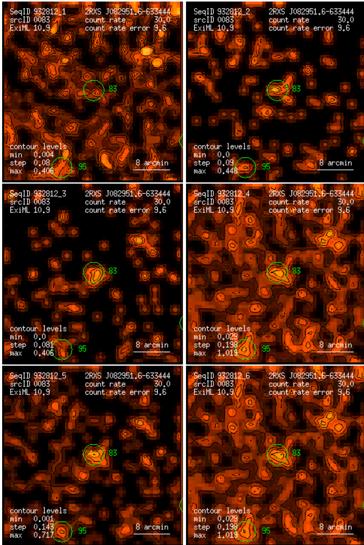
Figure 83: RASS 932812: detection 0083: band rate images, Gaussian filter: (1) PSPC channels 11 – 41, (2) 52 – 90, (3) 91 – 201, (4) 11 – 235, (5) 52 – 201, (6) 11 – 201. Broad band rates in counts/ks. Band rate contour levels in counts/ks/arcmin 2 .
