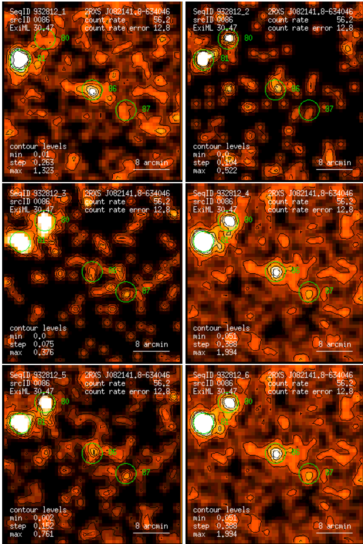
Figure 86: RASS 932812: detection 0086: band rate images, Gaussian filter: (1) PSPC channels 11 – 41, (2) 52 – 90, (3) 91 – 201, (4) 11 – 235, (5) 52 – 201, (6) 11 – 201. Broad band rates in counts/ks. Band rate contour levels in counts/ks/arcmin 2 .
