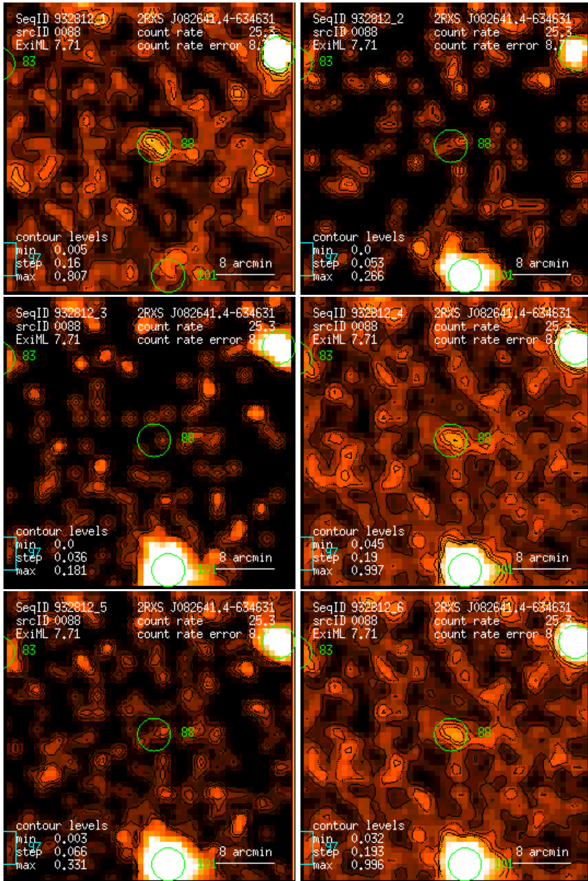
Figure 88: RASS 932812: detection 0088: band rate images, Gaussian filter: (1) PSPC channels 11 – 41, (2) 52 – 90, (3) 91 – 201, (4) 11 – 235, (5) 52 – 201, (6) 11 – 201. Broad band rates in counts/ks. Band rate contour levels in counts/ks/arcmin 2 .
