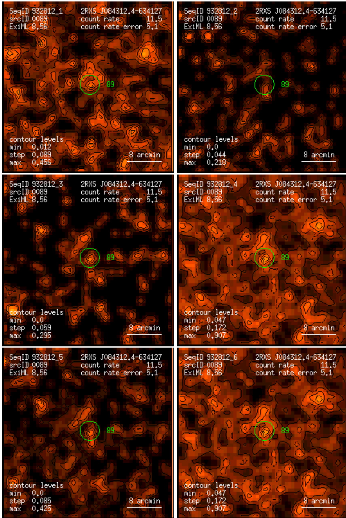
Figure 89: RASS 932812: detection 0089: band rate images, Gaussian filter: (1) PSPC channels 11 – 41, (2) 52 – 90, (3) 91 – 201, (4) 11 – 235, (5) 52 – 201, (6) 11 – 201. Broad band rates in counts/ks. Band rate contour levels in counts/ks/arcmin 2 .
