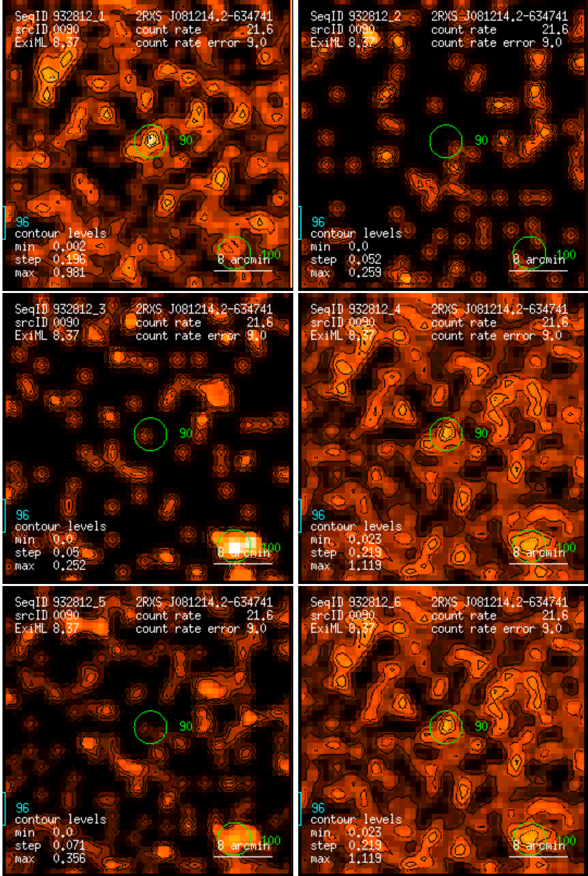
Figure 90: RASS 932812: detection 0090: band rate images, Gaussian filter: (1) PSPC channels 11 – 41, (2) 52 – 90, (3) 91 – 201, (4) 11 – 235, (5) 52 – 201, (6) 11 – 201. Broad band rates in counts/ks. Band rate contour levels in counts/ks/arcmin 2 .
