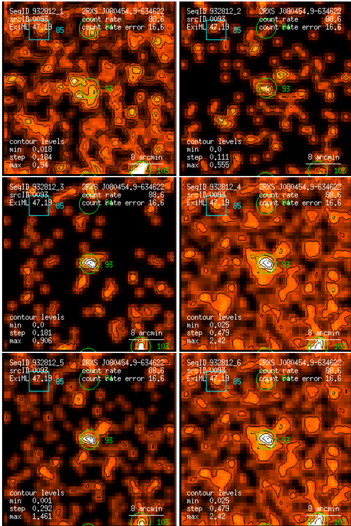
Figure 93: RASS 932812: detection 0093: band rate images, Gaussian filter: (1) PSPC channels 11 – 41, (2) 52 – 90, (3) 91 – 201, (4) 11 – 235, (5) 52 – 201, (6) 11 – 201. Broad band rates in counts/ks. Band rate contour levels in counts/ks/arcmin 2 .
