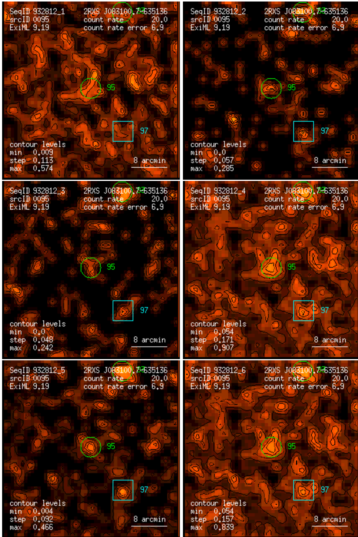
Figure 95: RASS 932812: detection 0095: band rate images, Gaussian filter: (1) PSPC channels 11 – 41, (2) 52 – 90, (3) 91 – 201, (4) 11 – 235, (5) 52 – 201, (6) 11 – 201. Broad band rates in counts/ks. Band rate contour levels in counts/ks/arcmin 2 .
