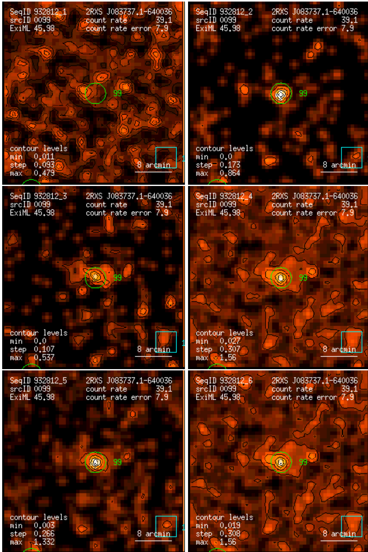
Figure 99: RASS 932812: detection 0099: band rate images, Gaussian filter: (1) PSPC channels 11 – 41, (2) 52 – 90, (3) 91 – 201, (4) 11 – 235, (5) 52 – 201, (6) 11 – 201. Broad band rates in counts/ks. Band rate contour levels in counts/ks/arcmin 2 .
