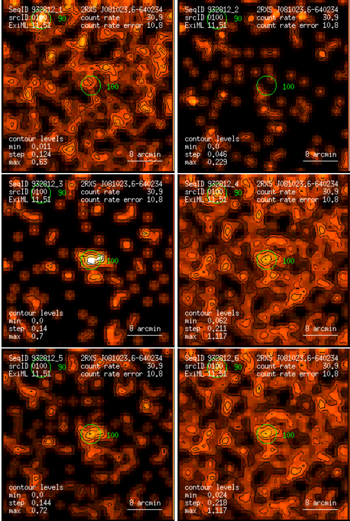
Figure 100: RASS 932812: detection 0100: band rate images, Gaussian filter: (1) PSPC channels 11 – 41, (2) 52 – 90, (3) 91 – 201, (4) 11 – 235, (5) 52 – 201, (6) 11 – 201. Broad band rates in counts/ks. Band rate contour levels in counts/ks/arcmin 2 .
