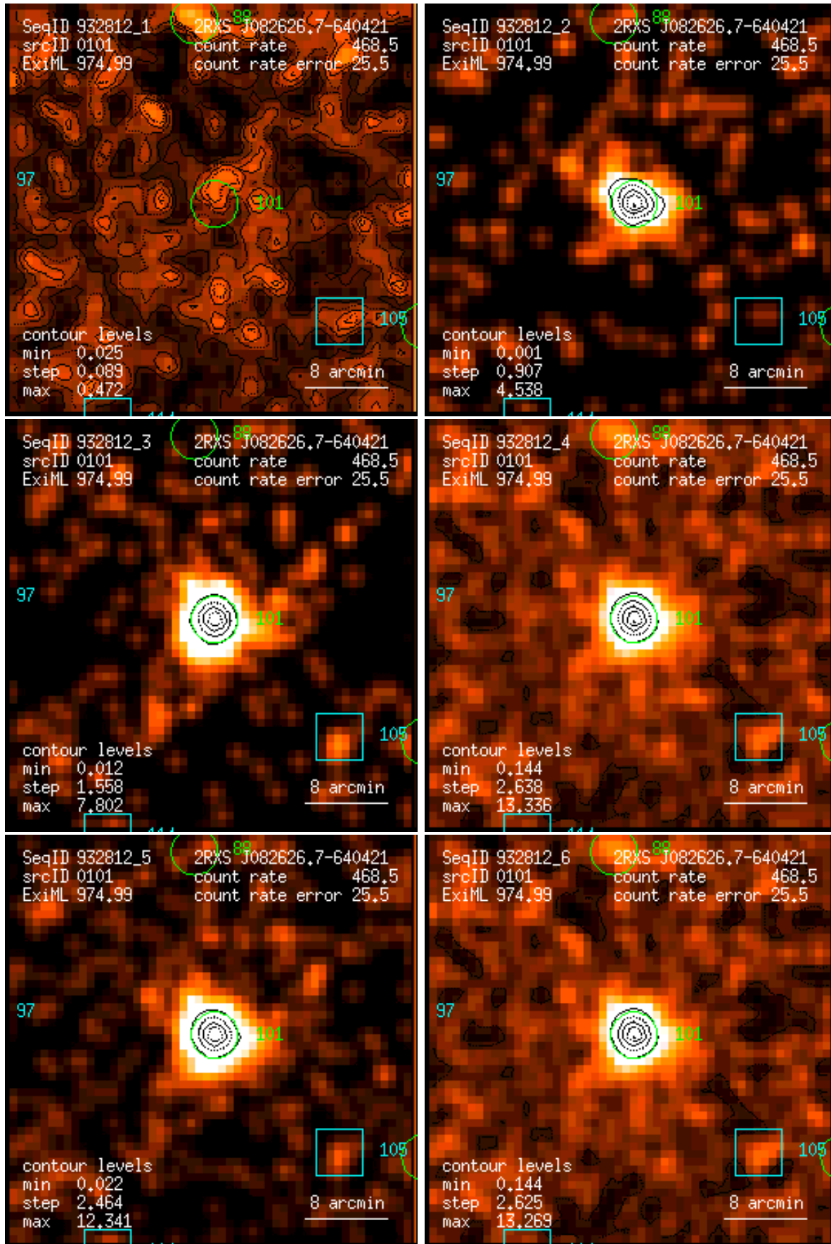
Figure 101: RASS 932812: detection 0101: band rate images, Gaussian filter: (1) PSPC channels 11 – 41, (2) 52 – 90, (3) 91 – 201, (4) 11 – 235, (5) 52 – 201, (6) 11 – 201. Broad band rates in counts/ks. Band rate contour levels in counts/ks/arcmin 2 .
