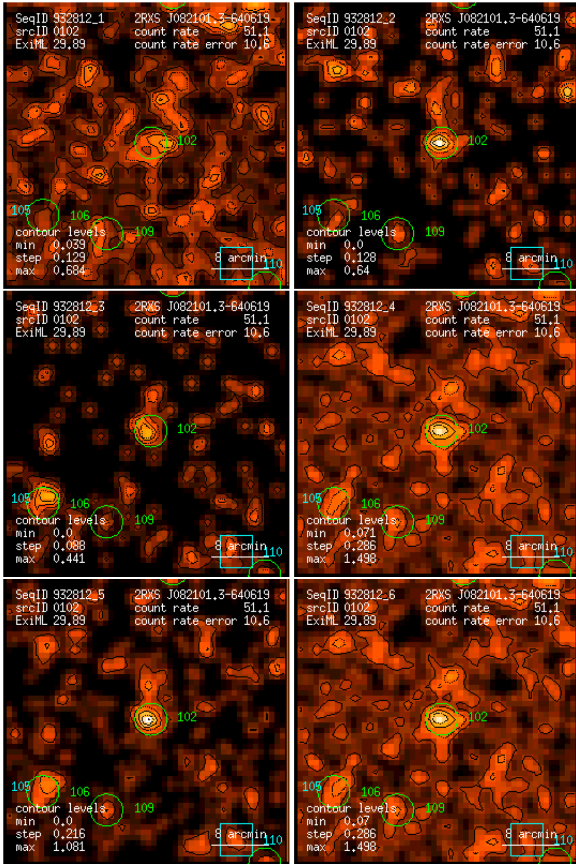
Figure 102: RASS 932812: detection 0102: band rate images, Gaussian filter: (1) PSPC channels 11 – 41, (2) 52 – 90, (3) 91 – 201, (4) 11 – 235, (5) 52 – 201, (6) 11 – 201. Broad band rates in counts/ks. Band rate contour levels in counts/ks/arcmin 2 .
