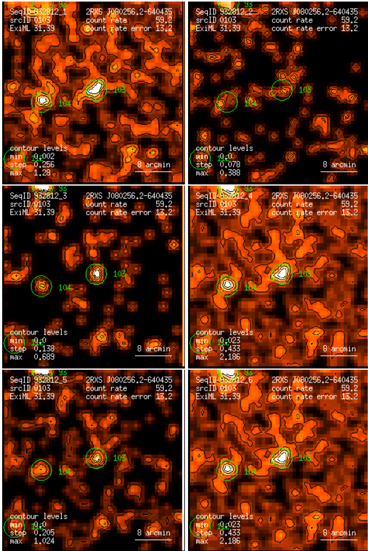
Figure 103: RASS 932812: detection 0103: band rate images, Gaussian filter: (1) PSPC channels 11 – 41, (2) 52 – 90, (3) 91 – 201, (4) 11 – 235, (5) 52 – 201, (6) 11 – 201. Broad band rates in counts/ks. Band rate contour levels in counts/ks/arcmin 2 .
