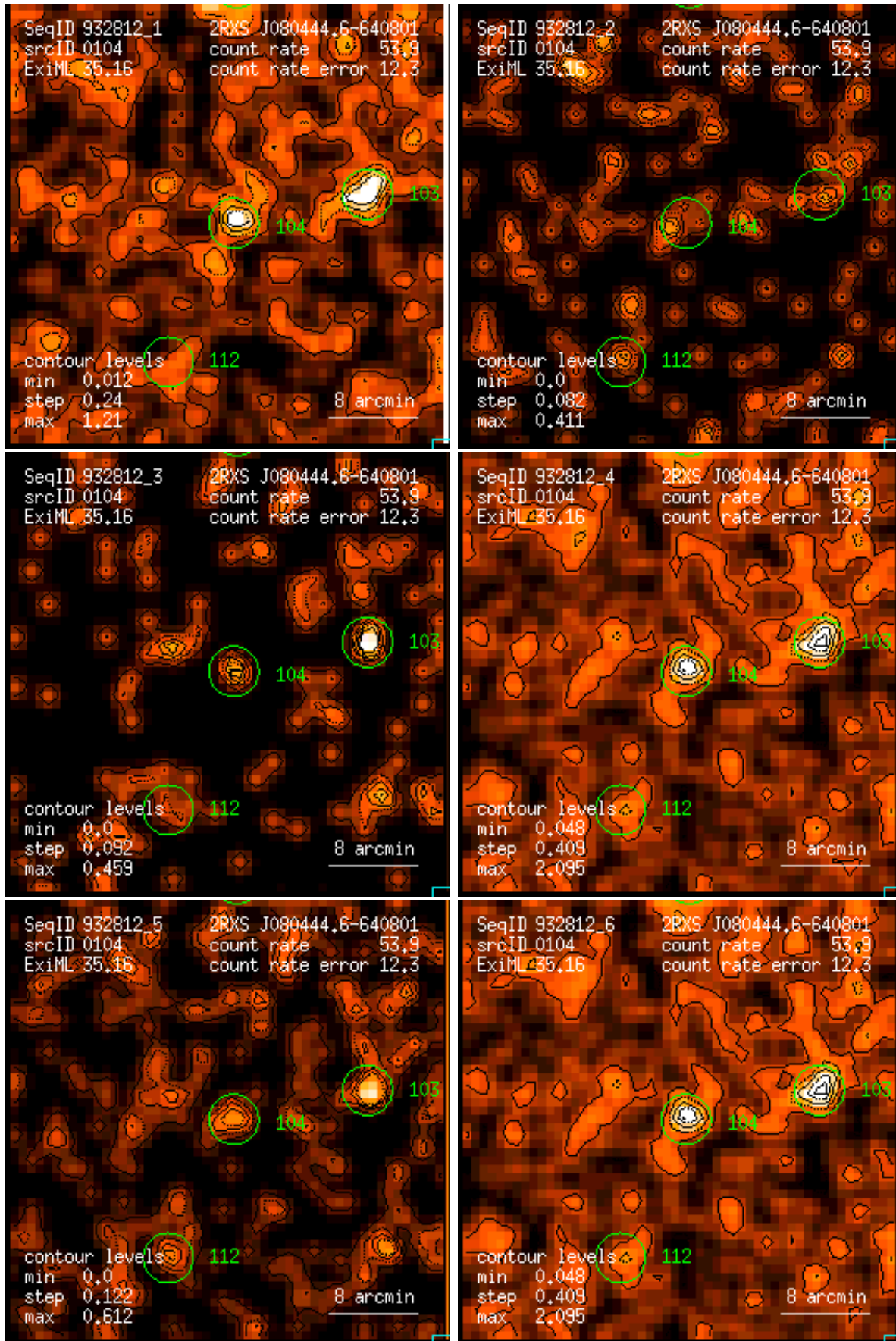
Figure 104: RASS 932812: detection 0104: band rate images, Gaussian filter: (1) PSPC channels 11 – 41, (2) 52 – 90, (3) 91 – 201, (4) 11 – 235, (5) 52 – 201, (6) 11 – 201. Broad band rates in counts/ks. Band rate contour levels in counts/ks/arcmin 2 .
