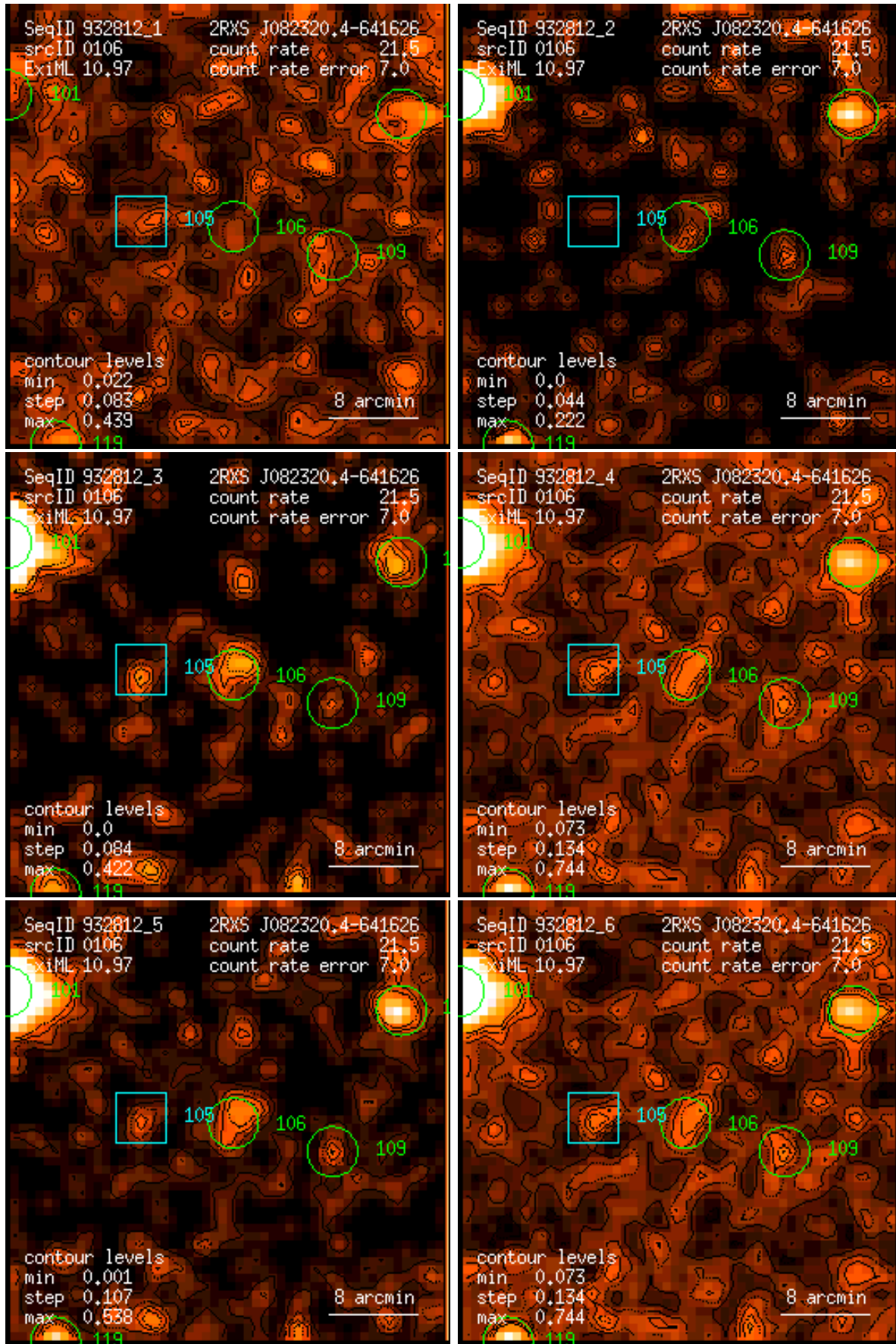
Figure 106: RASS 932812: detection 0106: band rate images, Gaussian filter: (1) PSPC channels 11 – 41, (2) 52 – 90, (3) 91 – 201, (4) 11 – 235, (5) 52 – 201, (6) 11 – 201. Broad band rates in counts/ks. Band rate contour levels in counts/ks/arcmin 2 .
