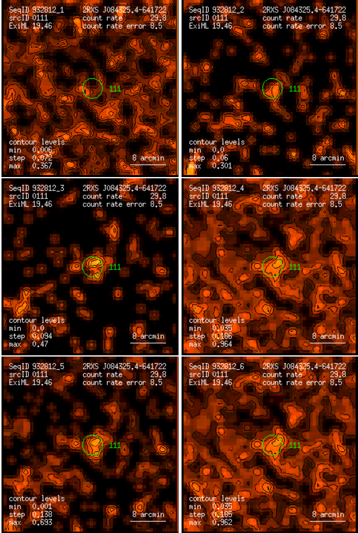
Figure 111: RASS 932812: detection 0111: band rate images, Gaussian filter: (1) PSPC channels 11 – 41, (2) 52 – 90, (3) 91 – 201, (4) 11 – 235, (5) 52 – 201, (6) 11 – 201. Broad band rates in counts/ks. Band rate contour levels in counts/ks/arcmin 2 .
