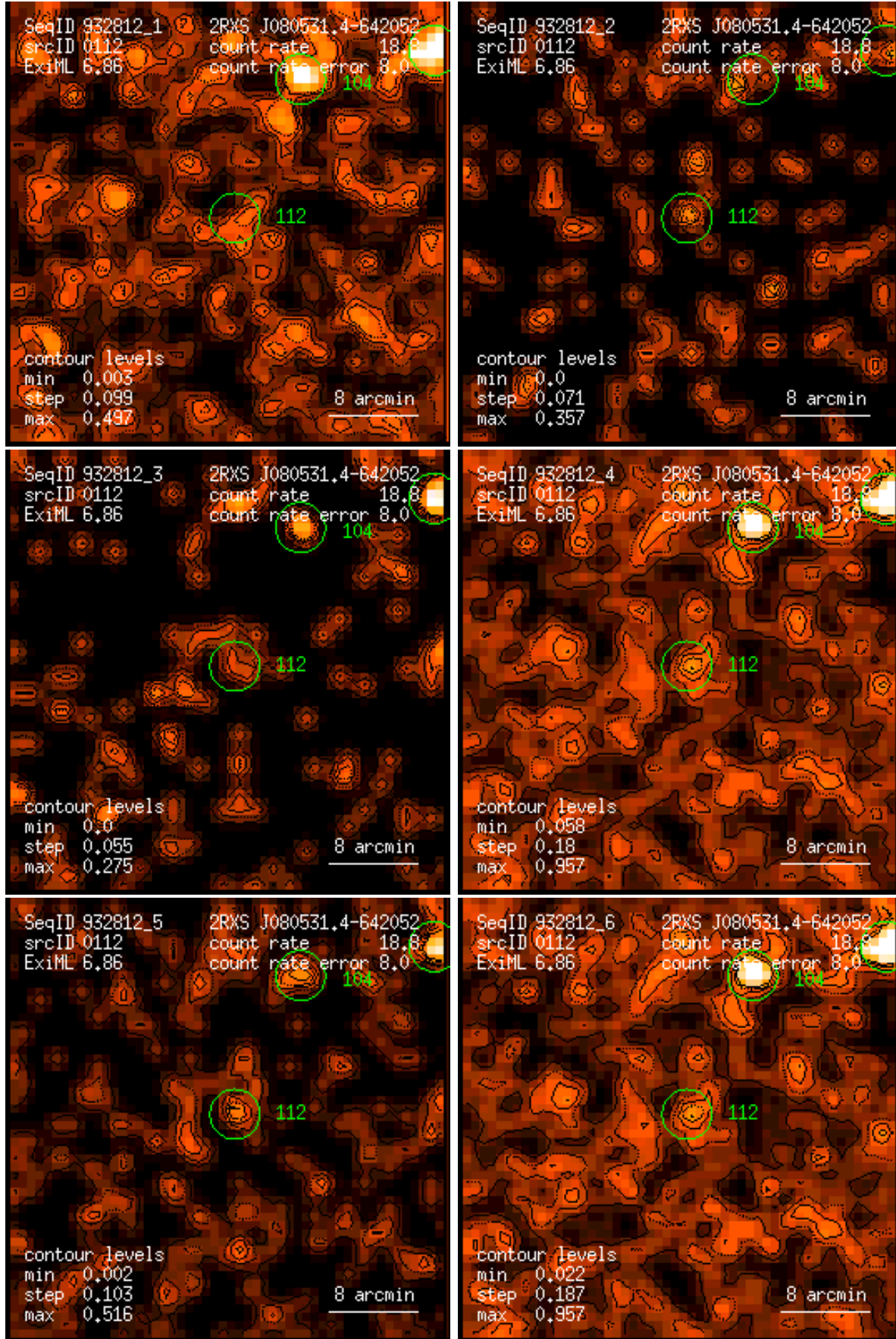
Figure 112: RASS 932812: detection 0112: band rate images, Gaussian filter: (1) PSPC channels 11 – 41, (2) 52 – 90, (3) 91 – 201, (4) 11 – 235, (5) 52 – 201, (6) 11 – 201. Broad band rates in counts/ks. Band rate contour levels in counts/ks/arcmin 2 .
