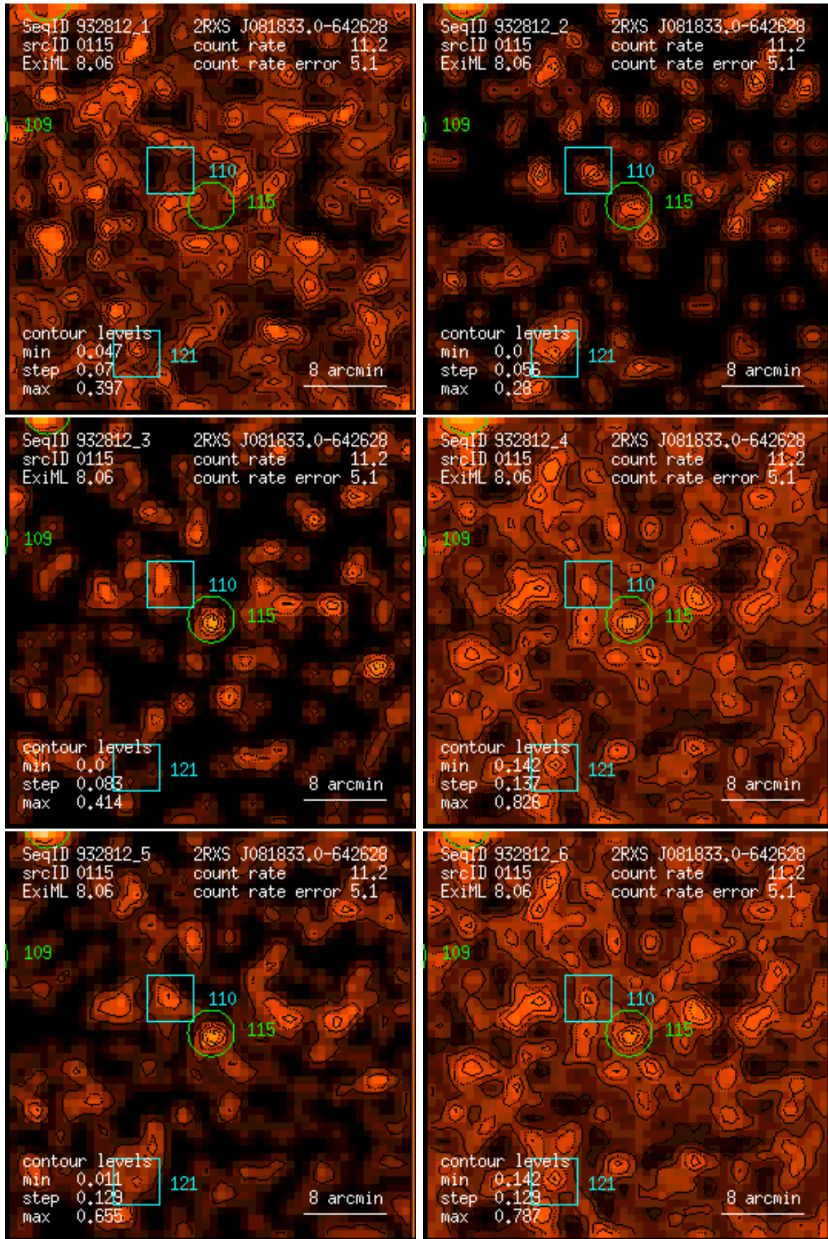
Figure 115: RASS 932812: detection 0115: band rate images, Gaussian filter: (1) PSPC channels 11 – 41, (2) 52 – 90, (3) 91 – 201, (4) 11 – 235, (5) 52 – 201, (6) 11 – 201. Broad band rates in counts/ks. Band rate contour levels in counts/ks/arcmin 2 .
